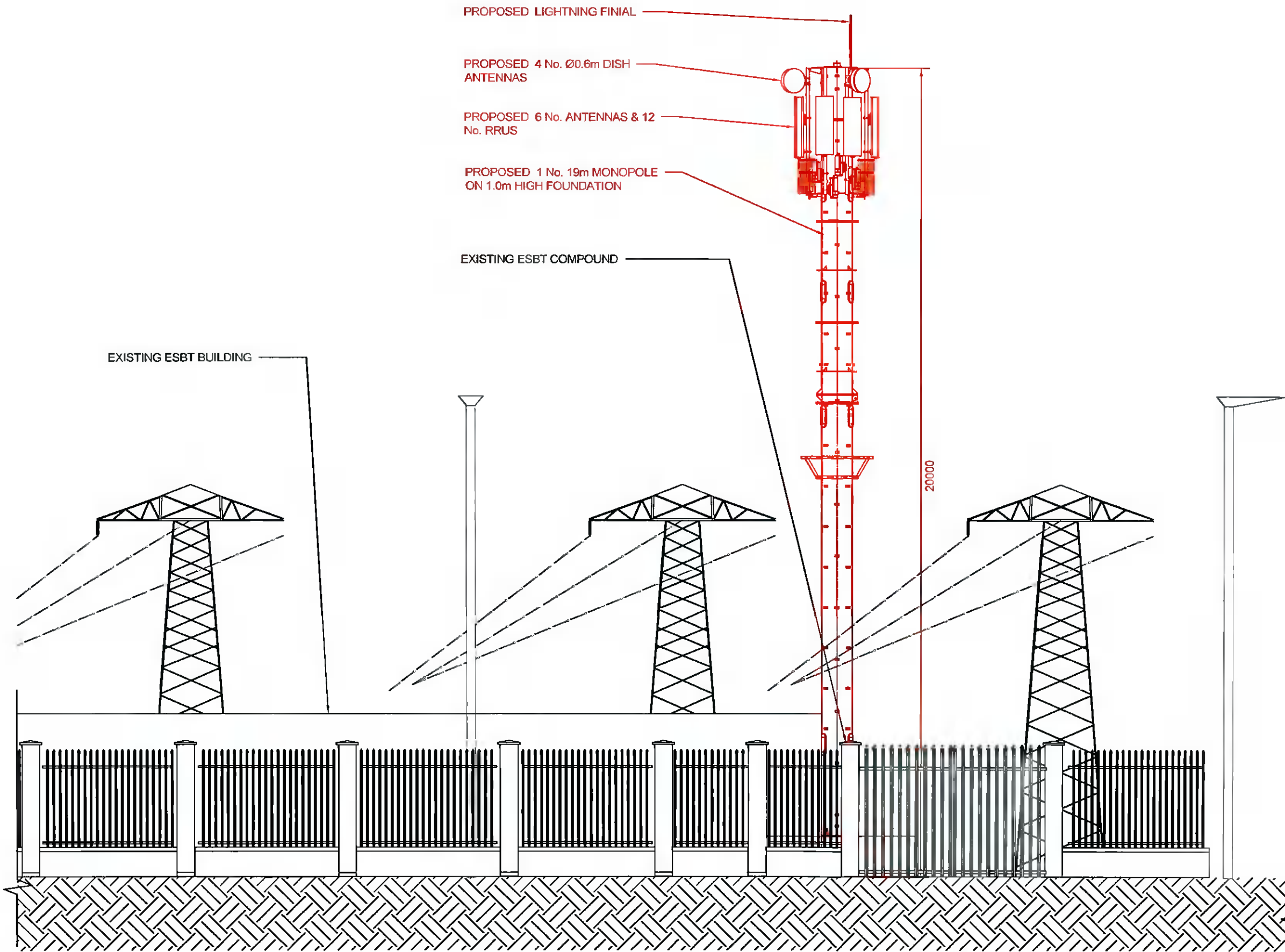
WEST ELEVATION 1/100 1/103
