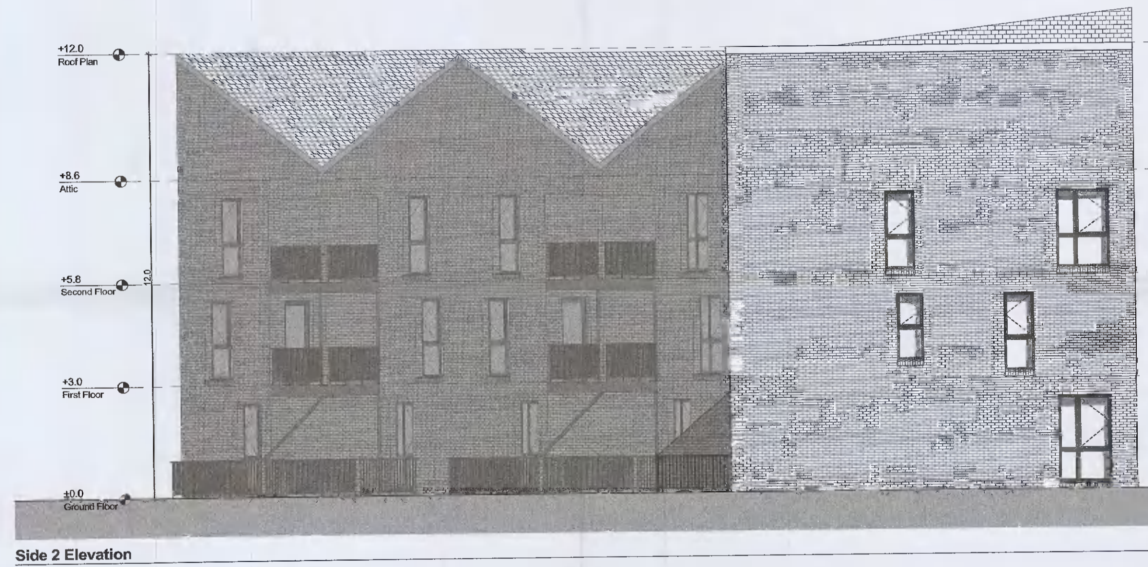
Side 2 Elevation
