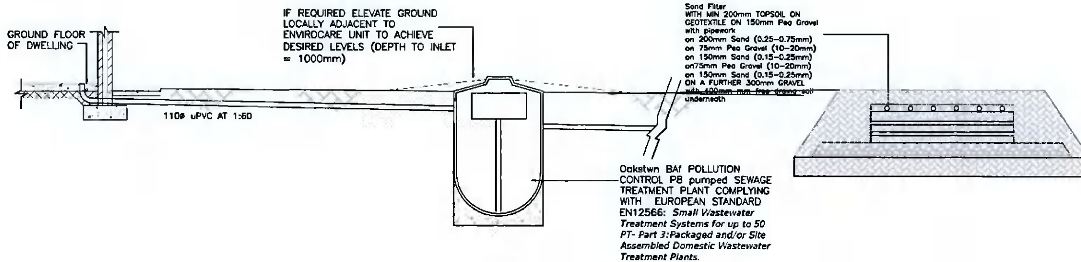
LONGITUDINAL SECTION THROUGH SYSTEM Scale 1:75
