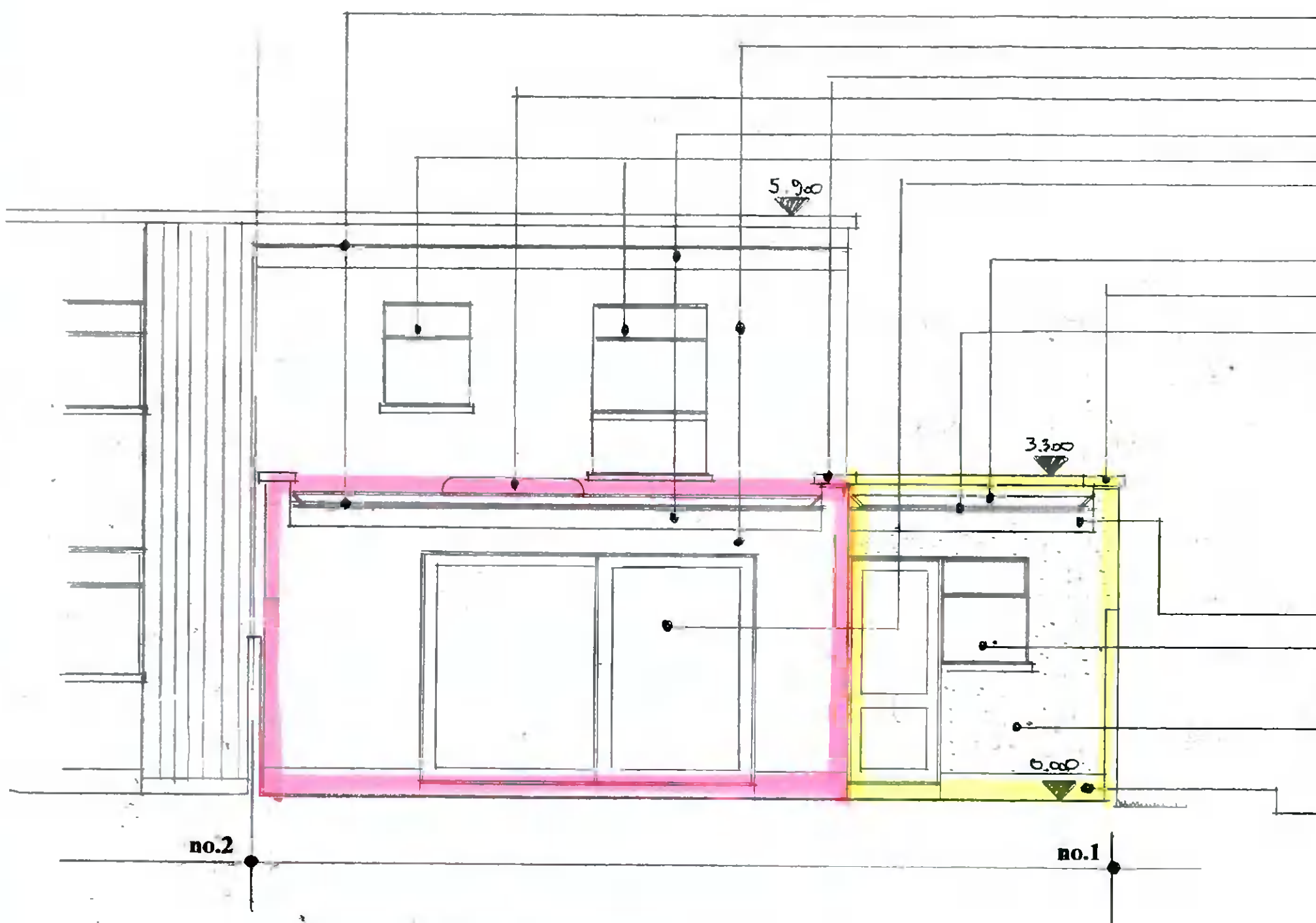
Proposed Rear Block Elevation Retention Rear Block Elevation scale 1:50.
