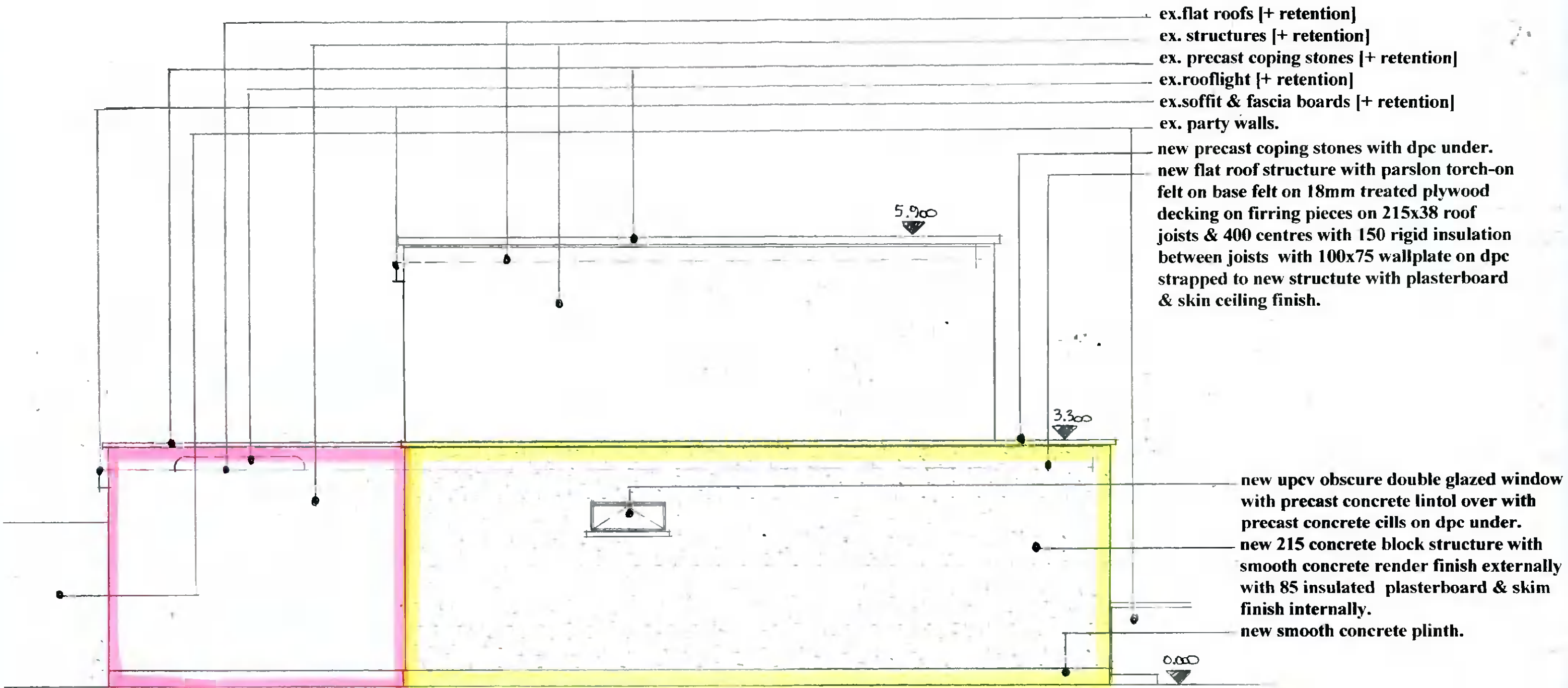
Proposed Side Elevation Retention Side Elevation scale 1:50.
