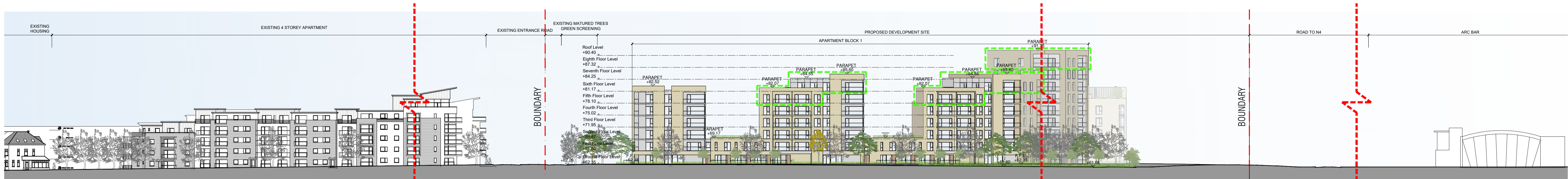
1- ELEVATION ALONG ST LOMAN'S ROAD SCALE 1:500
