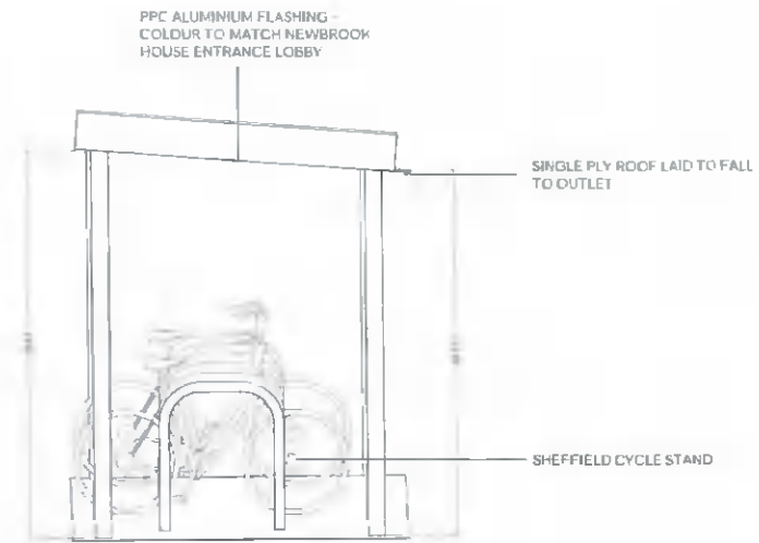
SIDE ELEVATION 1:50
