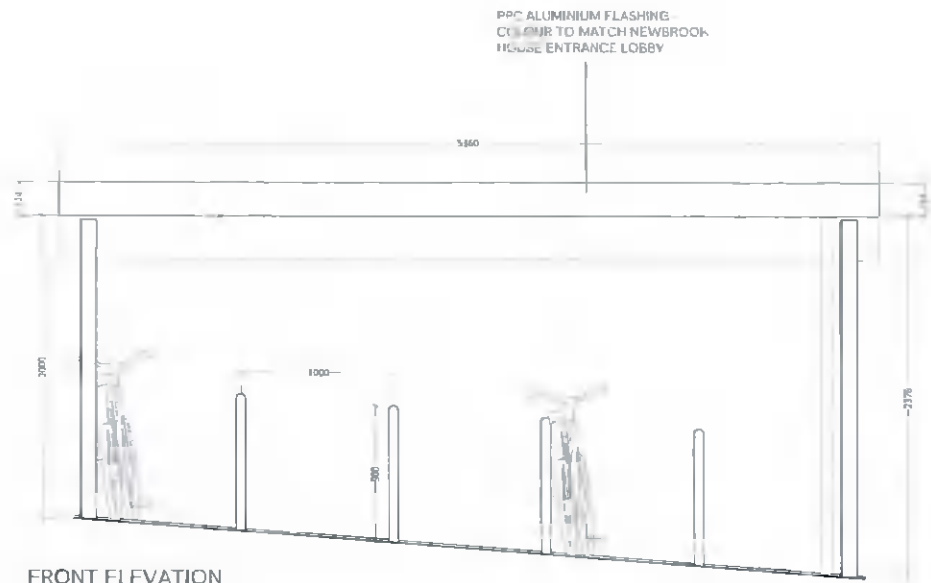
FRONT ELEVATION 1:50
