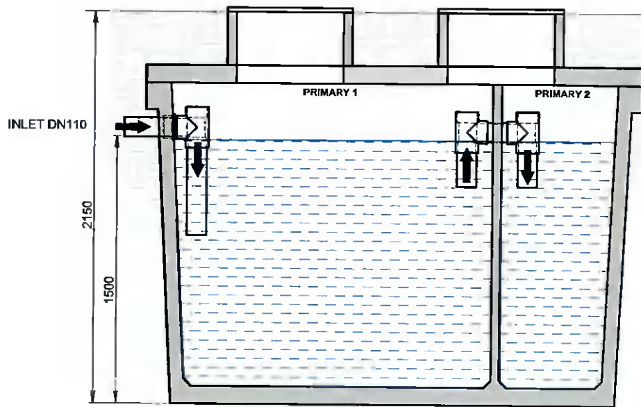
SECTION B-B
