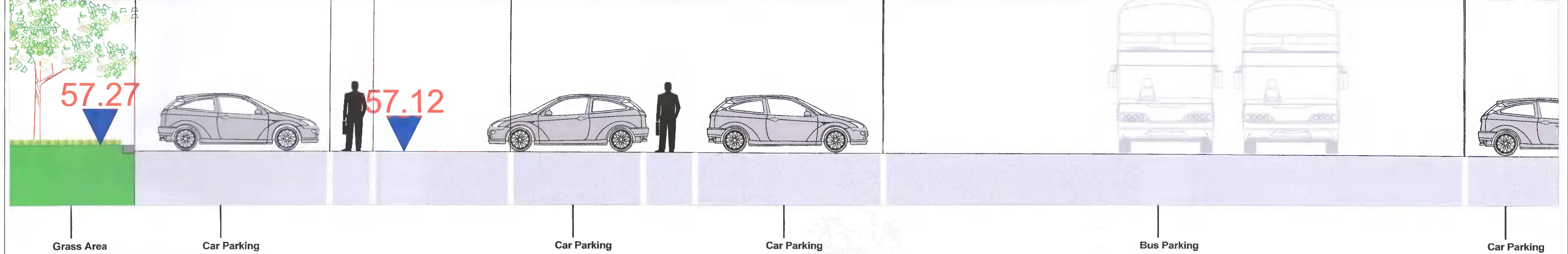
Detail 2 Existing Section B - BB scale 1:50
