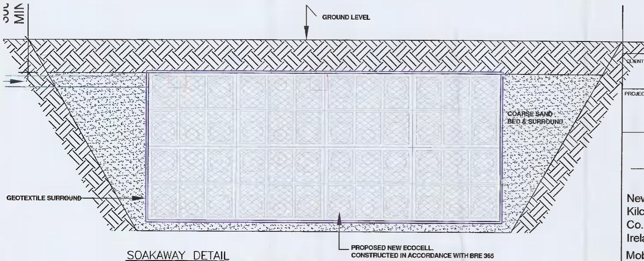
SOAKAWAY DETAIL
