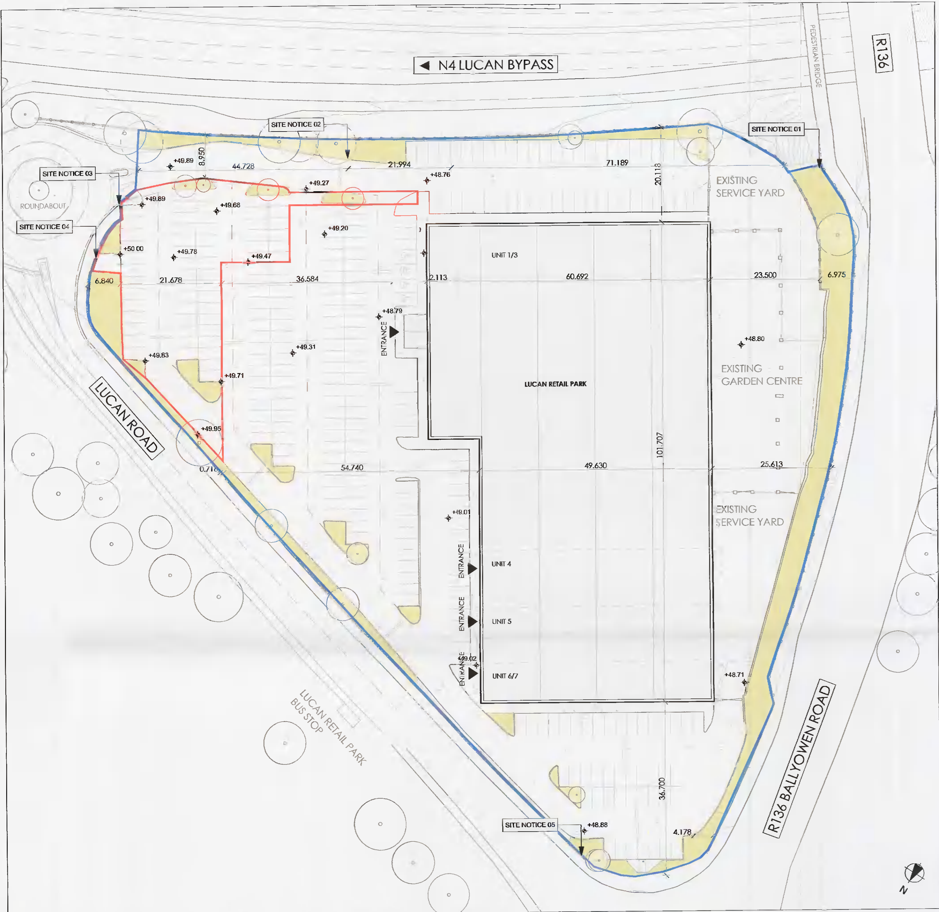
Existing Site Plan 1:500
