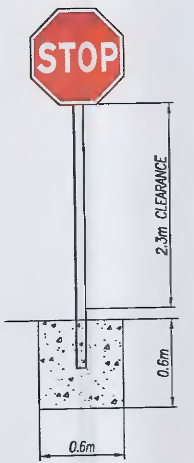
POLE DETAIL NTS
