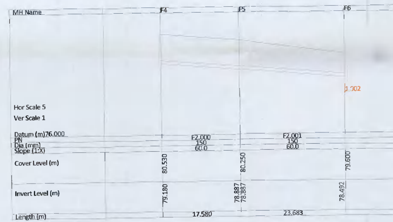
WASTEWATER NETWORK F2.000 - F2.001
