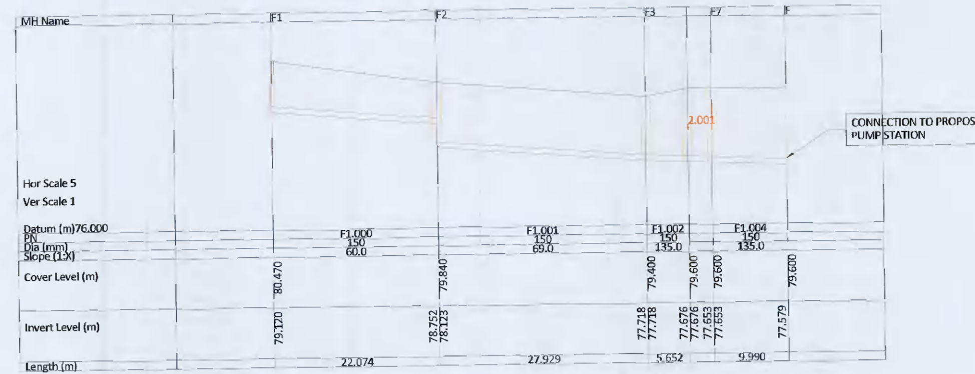
WASTEWATER NETWORK F1.000 - F1.004
