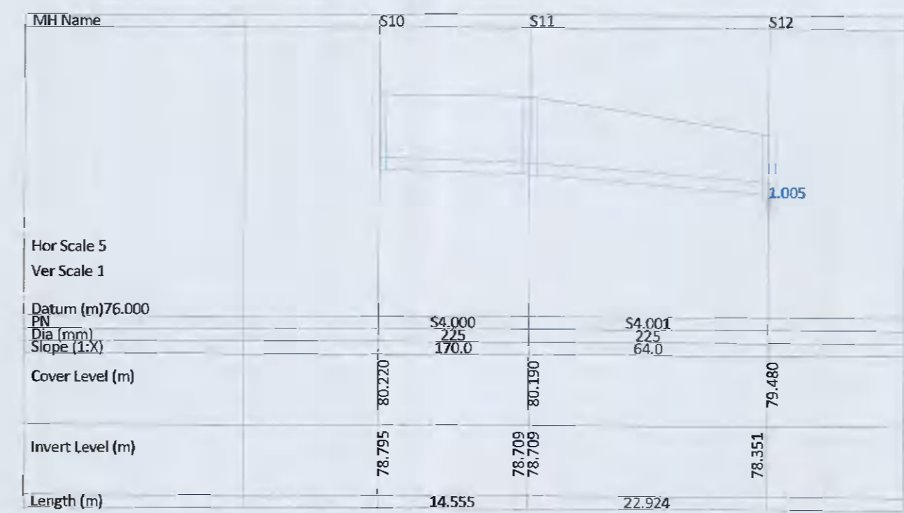
SURFACE WATER NETWORK S4.000-S4.001
