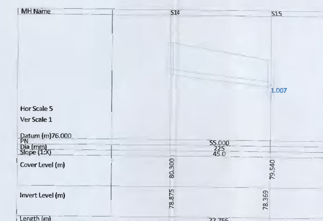
SURFACE WATER NETWORK S5.000
