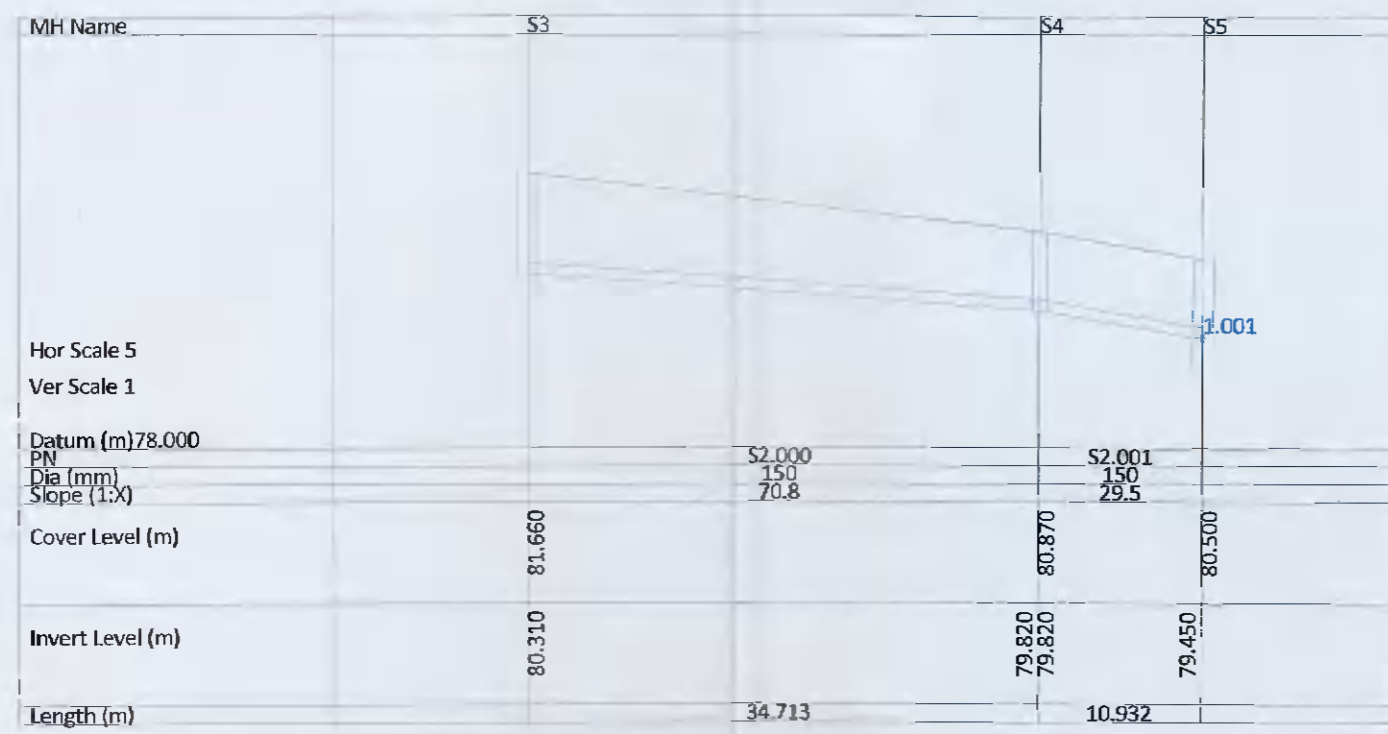
SURFACE WATER NETWORK S2.000 - S2.001
