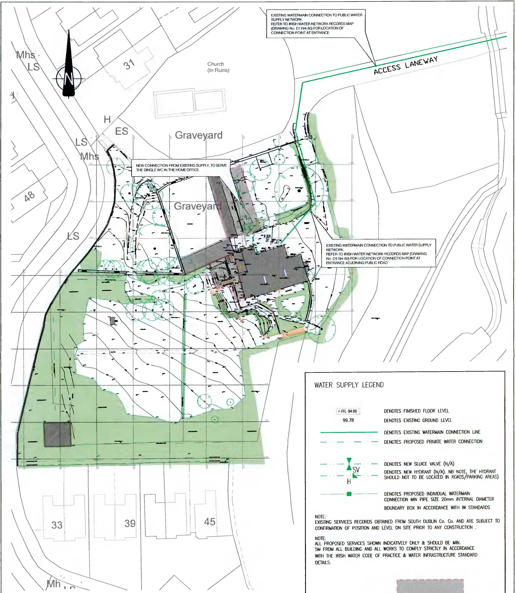
EXISTING/ PROPOSED WATERMAIN LAYOUT PLAN SCALE 1:500 FOR PLANNING PURPOSES ONLY
