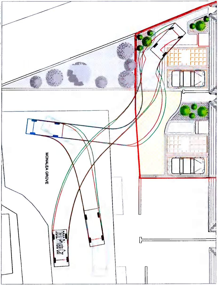
Vehicle Tracking 1 - Driving in and reverse exiting SCALE 1:200
