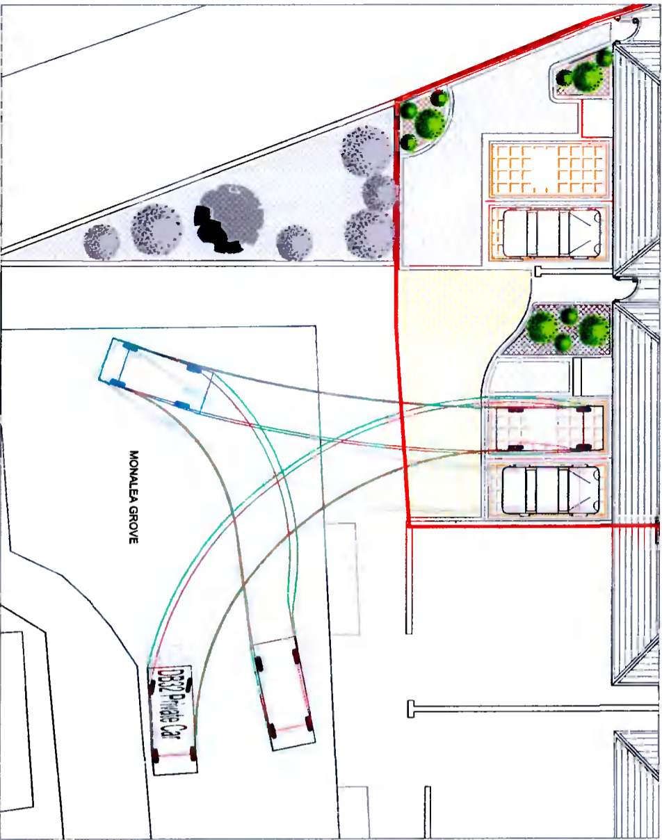
Vehicle Tracking 3 - Driving in and reverse exiting SCALE 1:200
