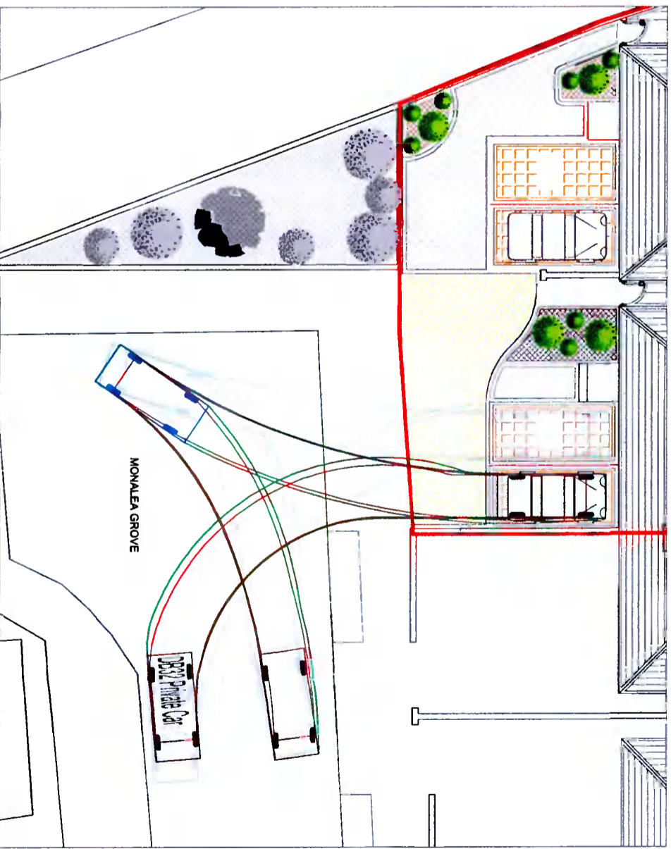
Vehicle Tracking 4 - Driving in and reverse exiting SCALE 1:200
