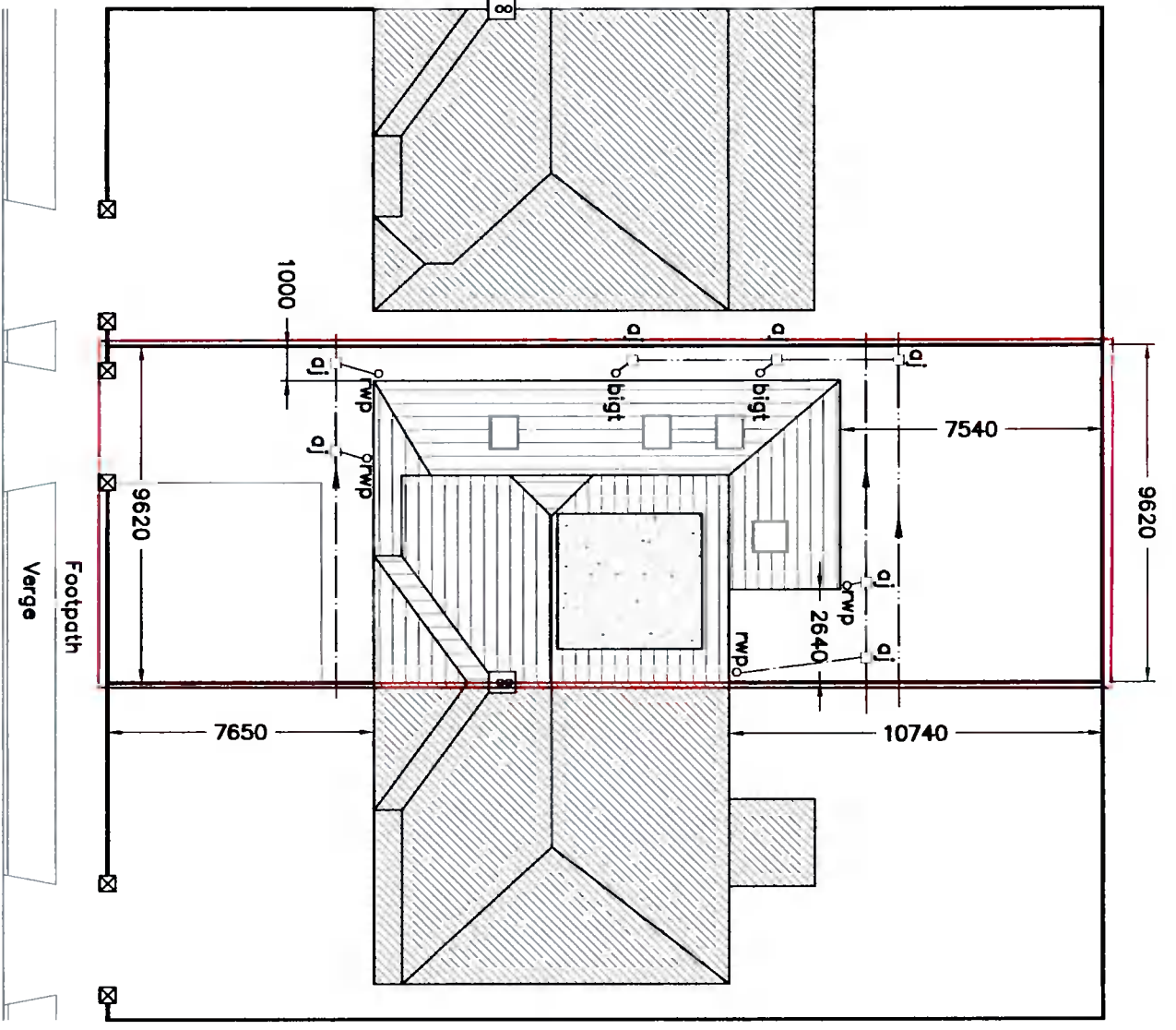
Proposed Block Plan & Drainage Layout SCALE 1:200
