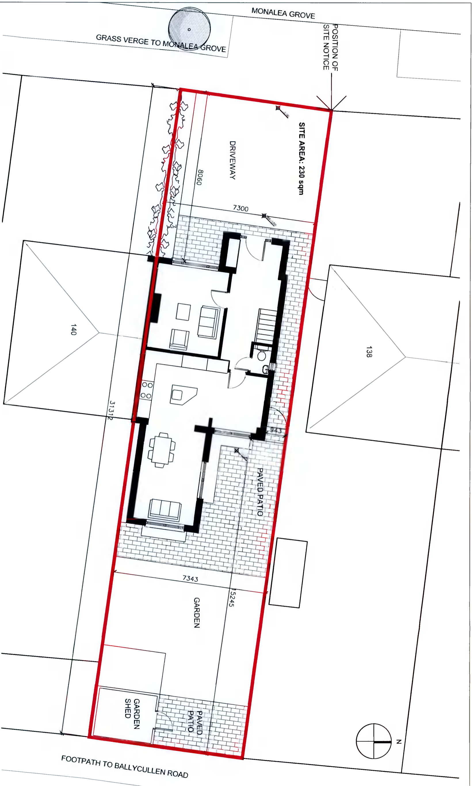
1 Site Layout Plan Scale 1:100 @ A3
