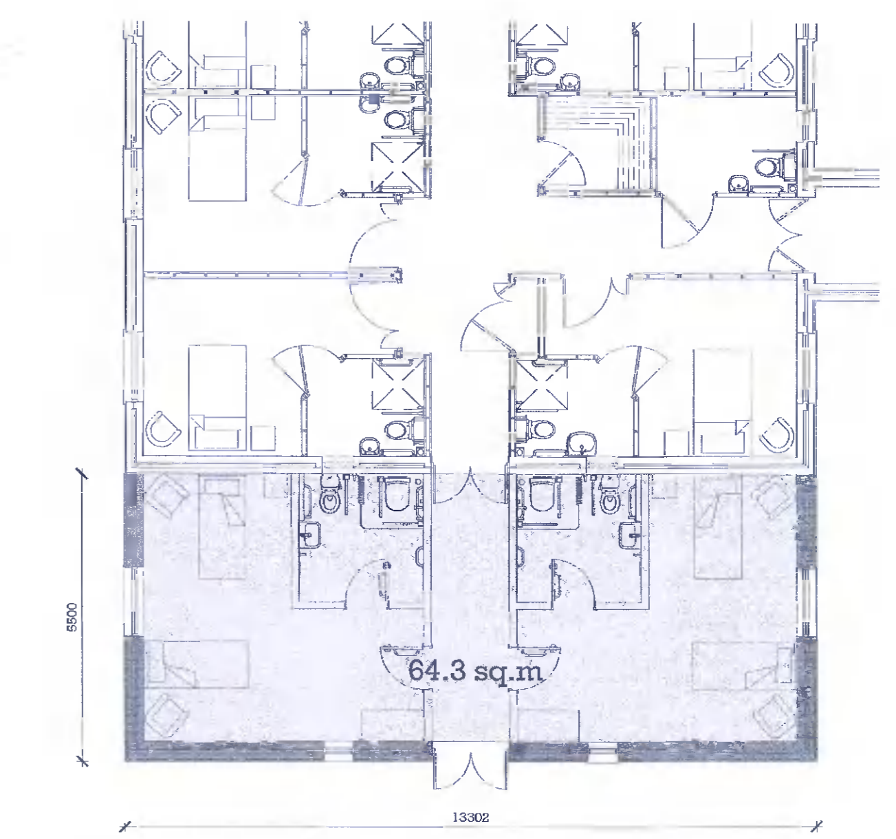
02 GROUND FLOOR B SCALE: 1:100
