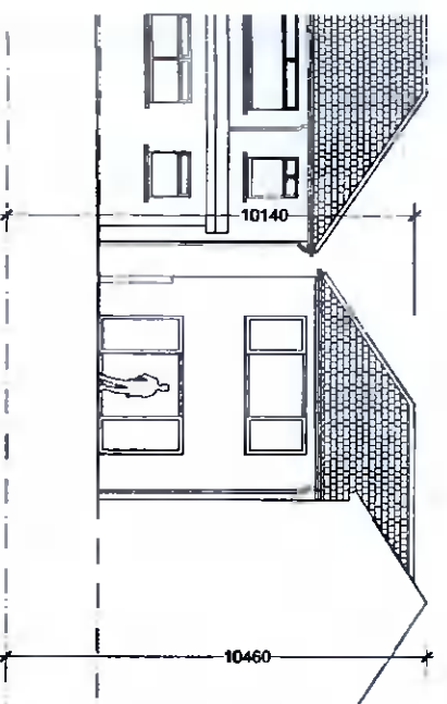
ELEVATION D SCALE 1:200@A3
