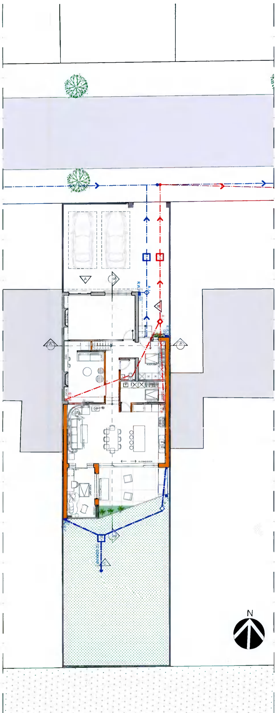
02 PROPOSED DRAINAGE PLAN SCALE: 1:200
