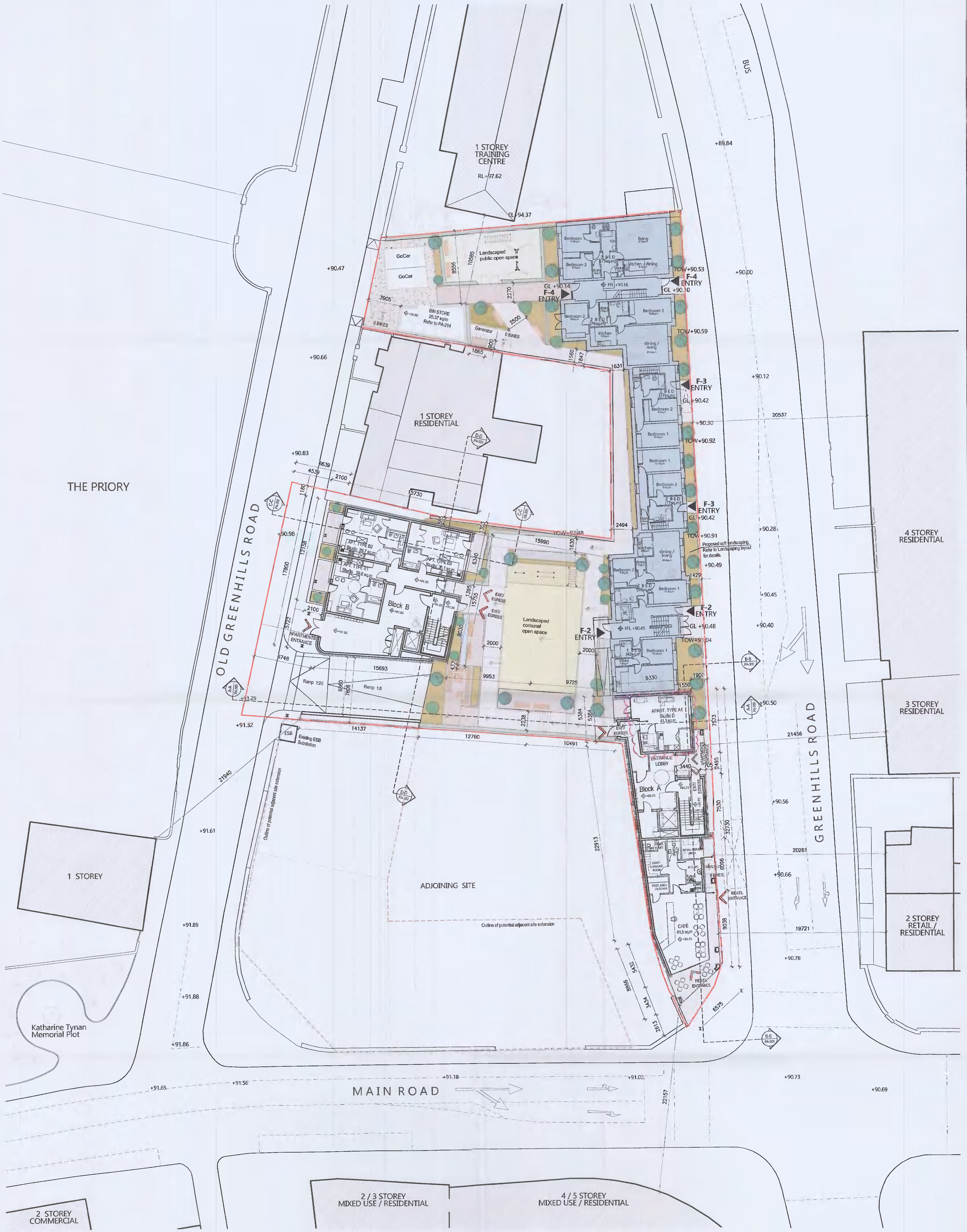
1 PROPOSED GROUND FLOOR PLAN AI-207 Scale: 1:200
