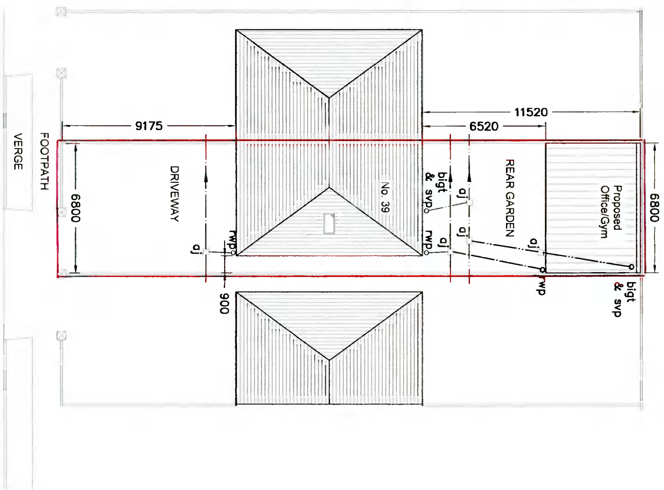
Proposed Block Plan & Drainage Layout SCALE 1:200
