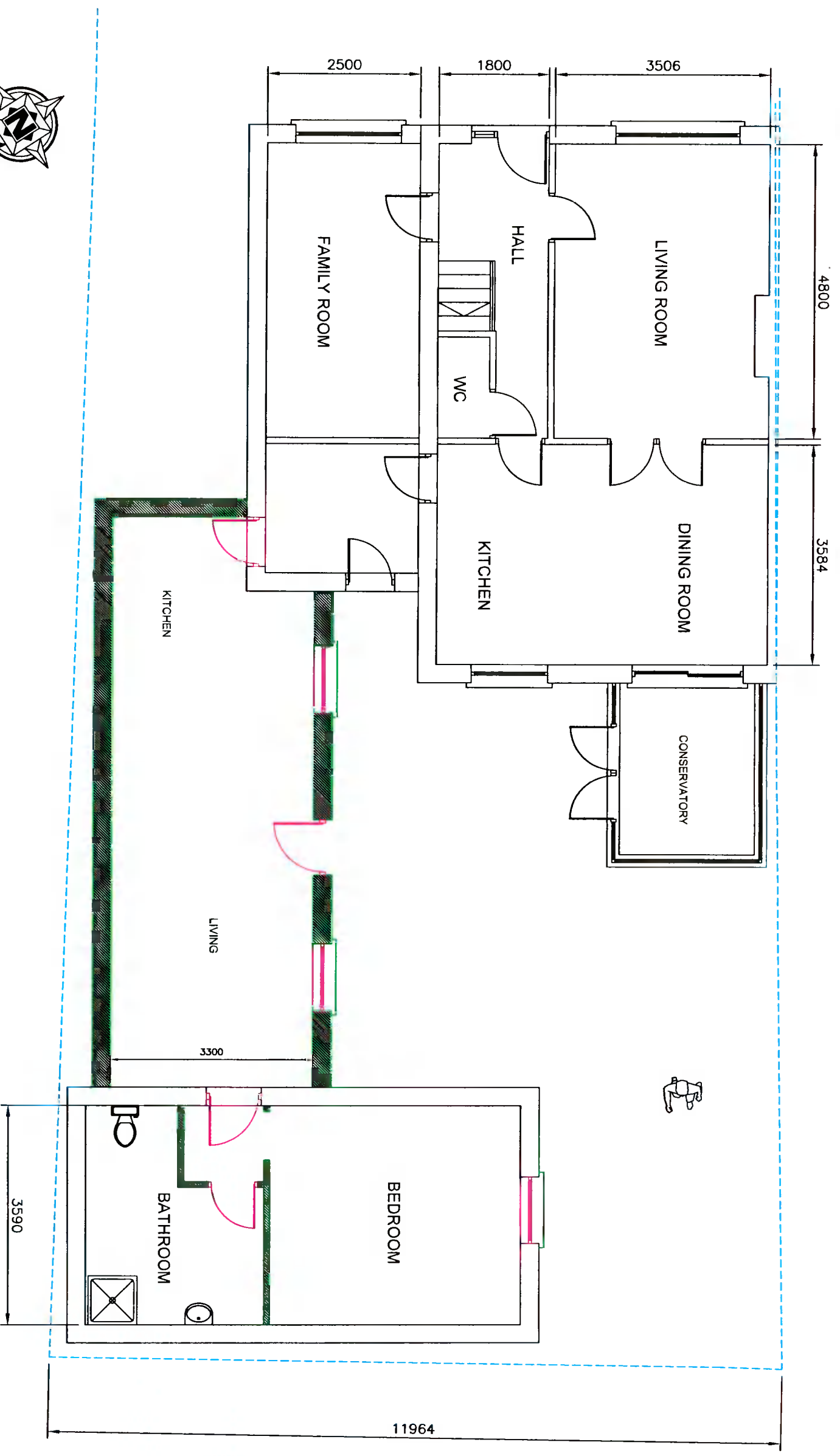
PROPOSED GROUND FLOOR PLAN VIEW
