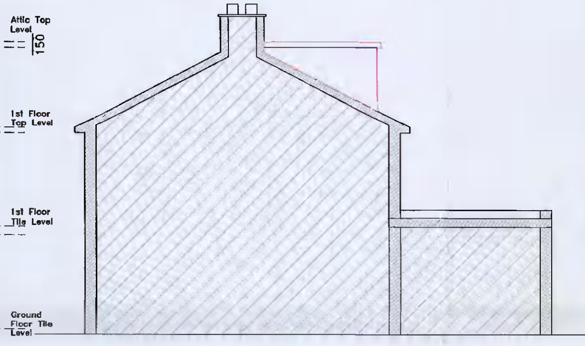
SIDE ELEVATION (EAST) (EXISTING & PROPOSED) SCALE 1:100
