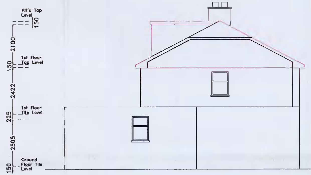
SIDE ELEVATION (WEST) (EXISTING & PROPOSED) SCALE 1:100
