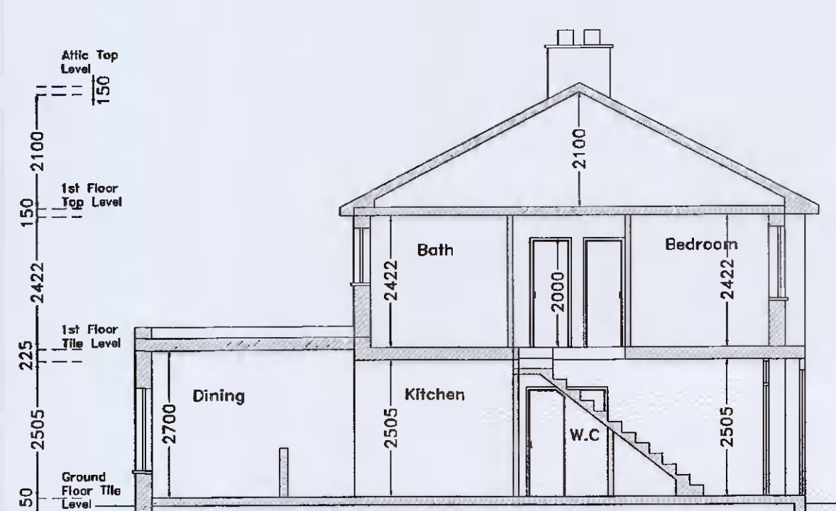
SECTION A-A (EXISTING) SCALE 1:100
