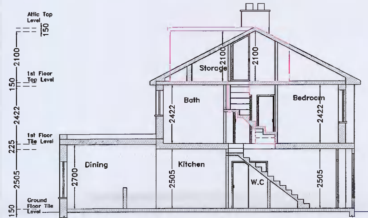
SECTION A-A (EXISTING & PROPOSED) SCALE 1:100
