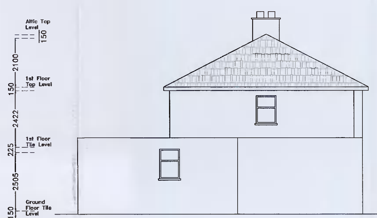
SIDE ELEVATION (WEST) (EXISTING) SCALE 1:100
