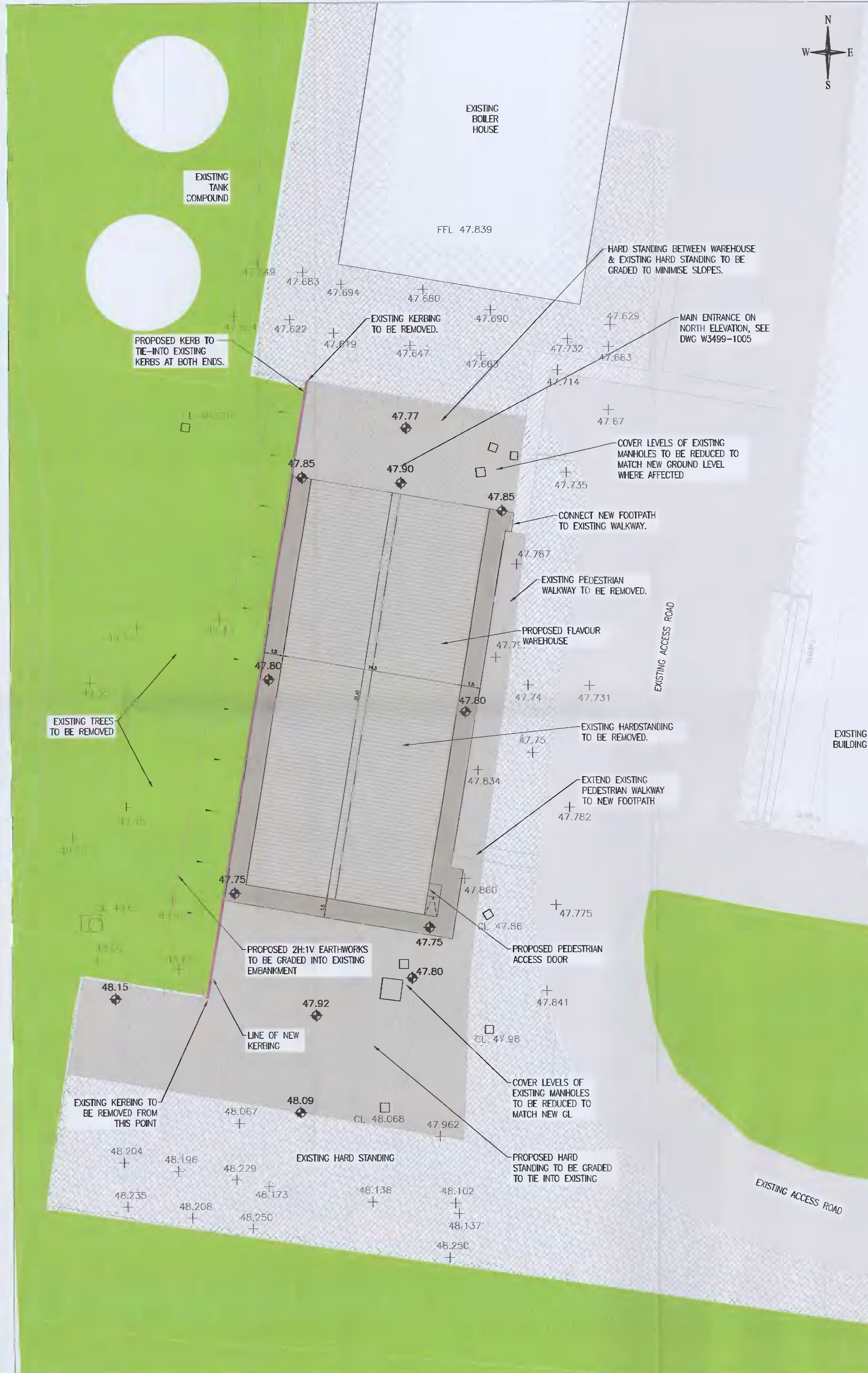
PROPOSED SITE FINISHES - FLAVOUR WAREHOUSE SCALE 1:200
