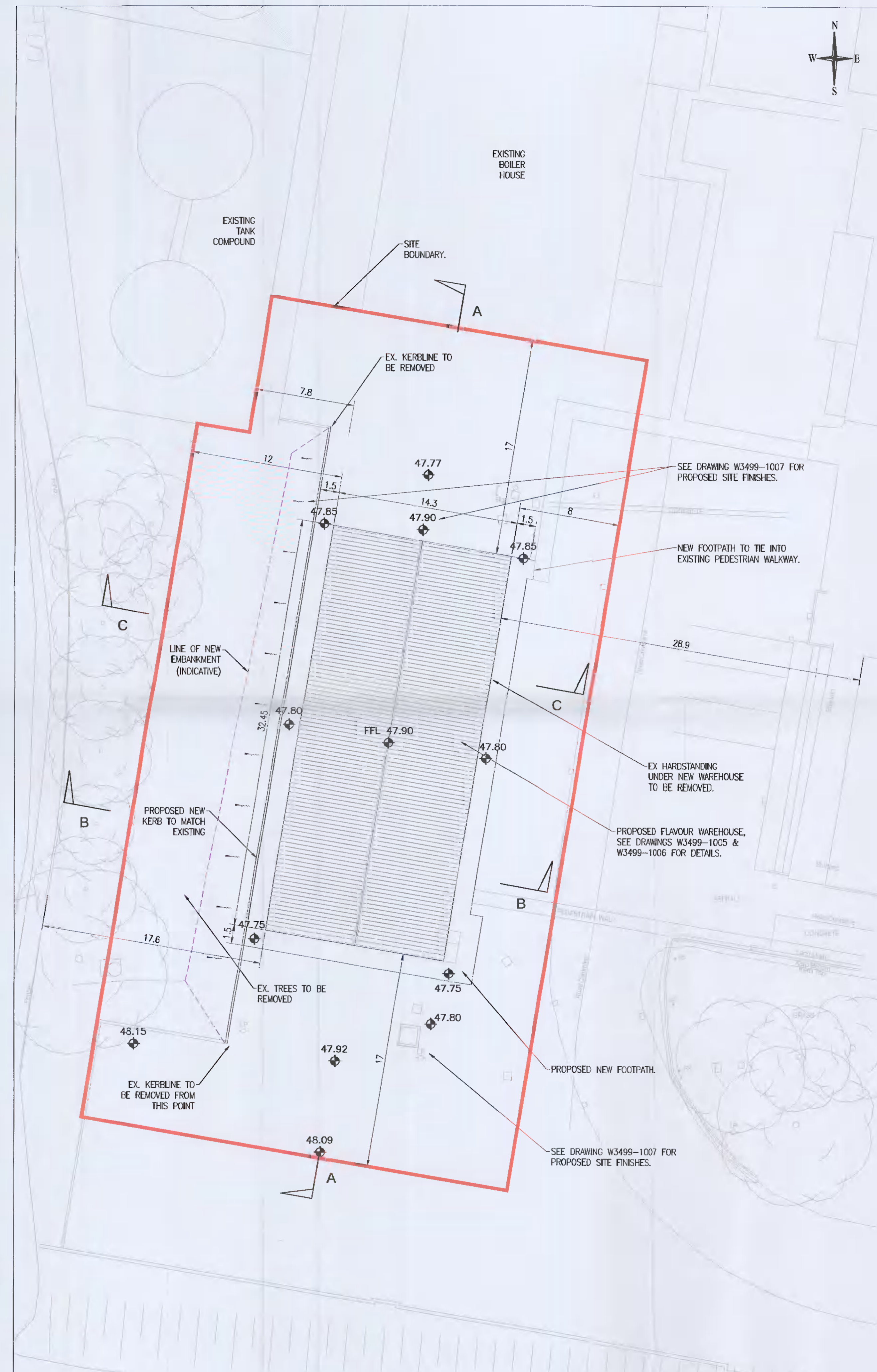
PROPOSED SITE LAYOUT PLAN - FLAVOUR WAREHOUSE SCALE 1:200
