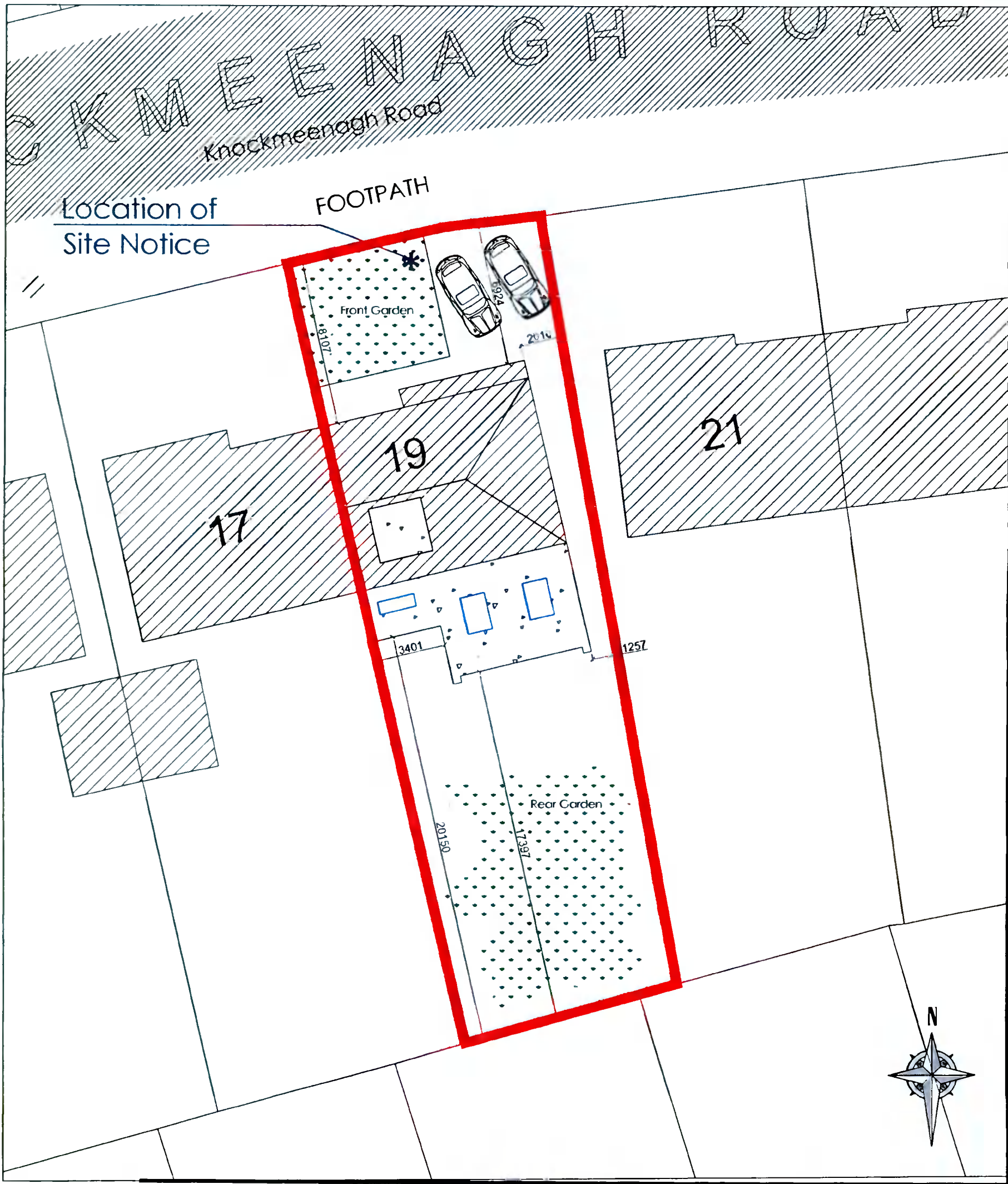
Proposed Site Layout Plan Scale: 1/200
