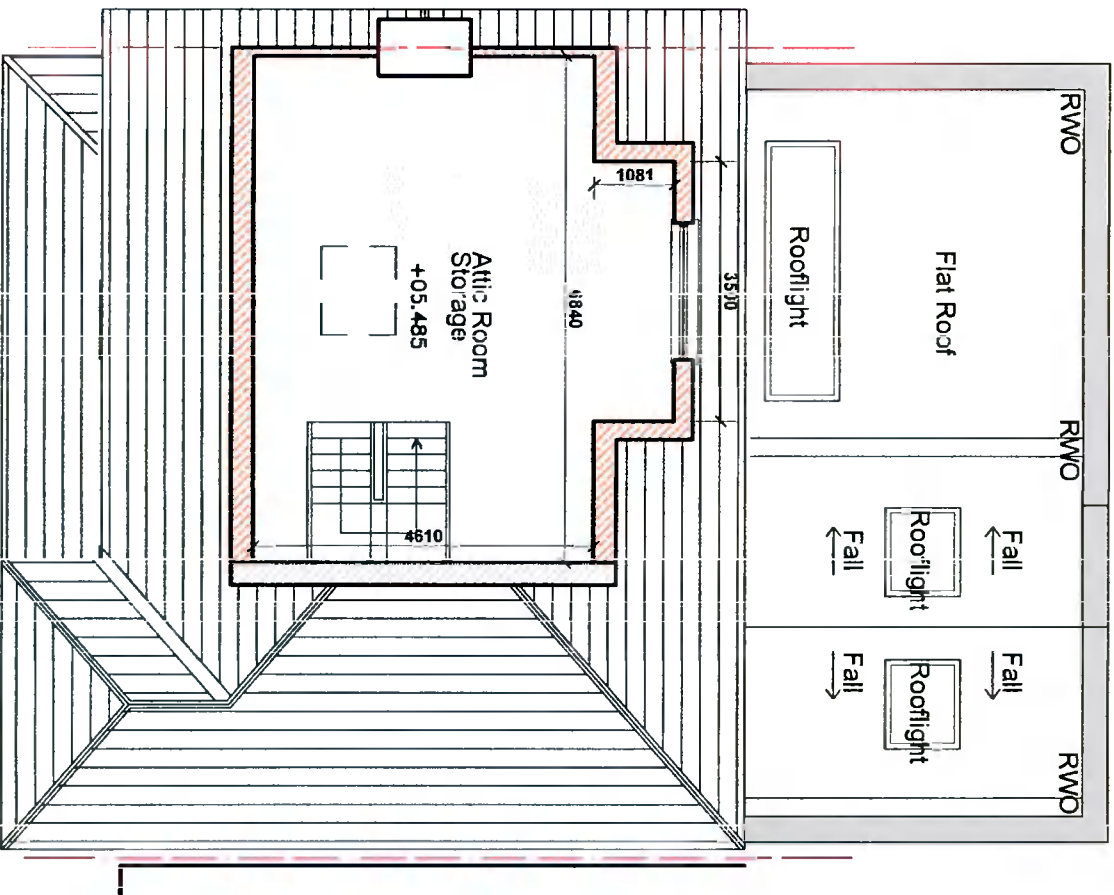
Proposed Attic Plan Scale 1/100
