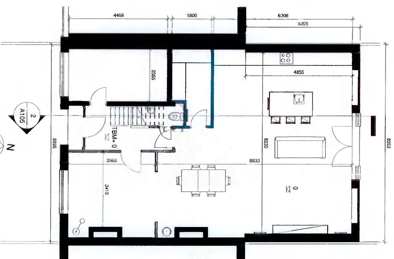
2. Existing Ground 1 : 100
