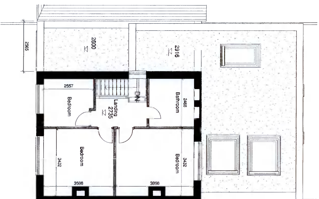
1. Existing First Floor 1 : 100
