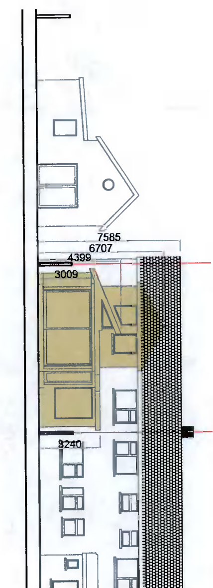
Proposed Rear Contiguous Elevation 1:200
