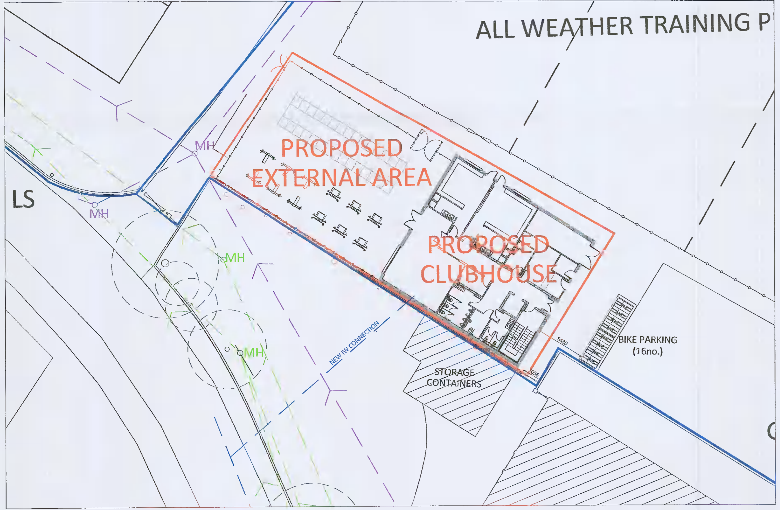
3 Proposed Site Layout - Revised For Additional Information scale 1:250 @ A1 Site Boundary Outlined in Red Lands under Management Licence Drainage - Mains Foul Drainage - Mains Surface Mains Water (Irish Water)
