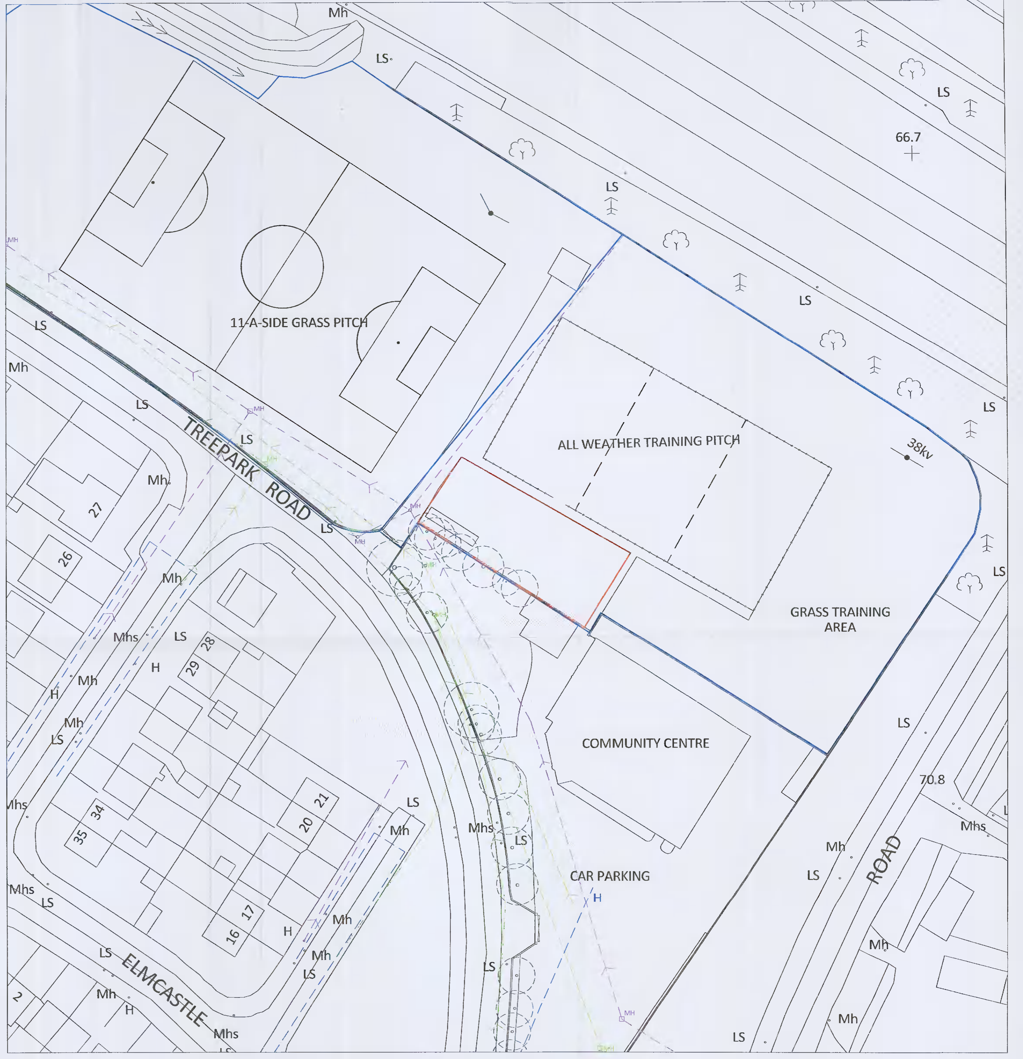
2 Existing Site Layout scale 1:500 @ A1 Site Boundary Outlined in Red Lands under Management Licence Drainage - Mains Foul Drainage - Mains Surface Mains Water (Irish Water)
