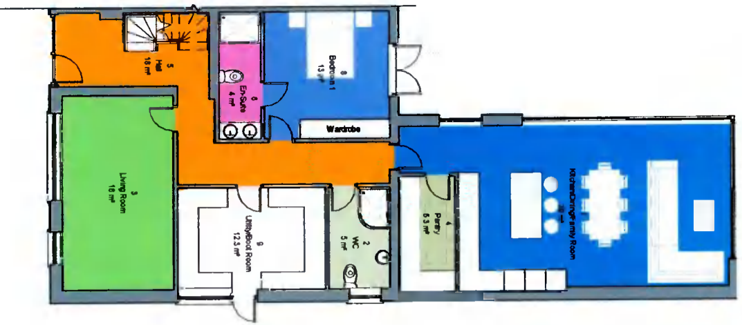
1 Level 0 Ground Floor Proposed Colour Fill 1 : 150
