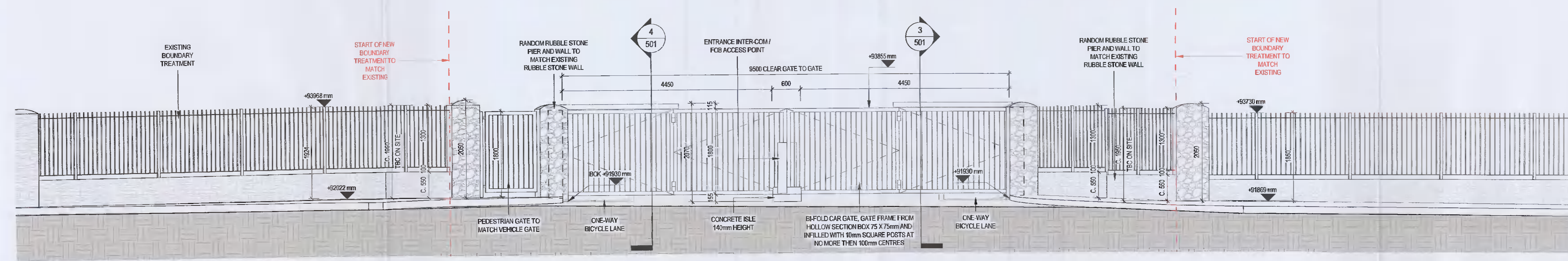
2 Proposed Pedestrian Gate Elevation - Front Scale: 1:50
