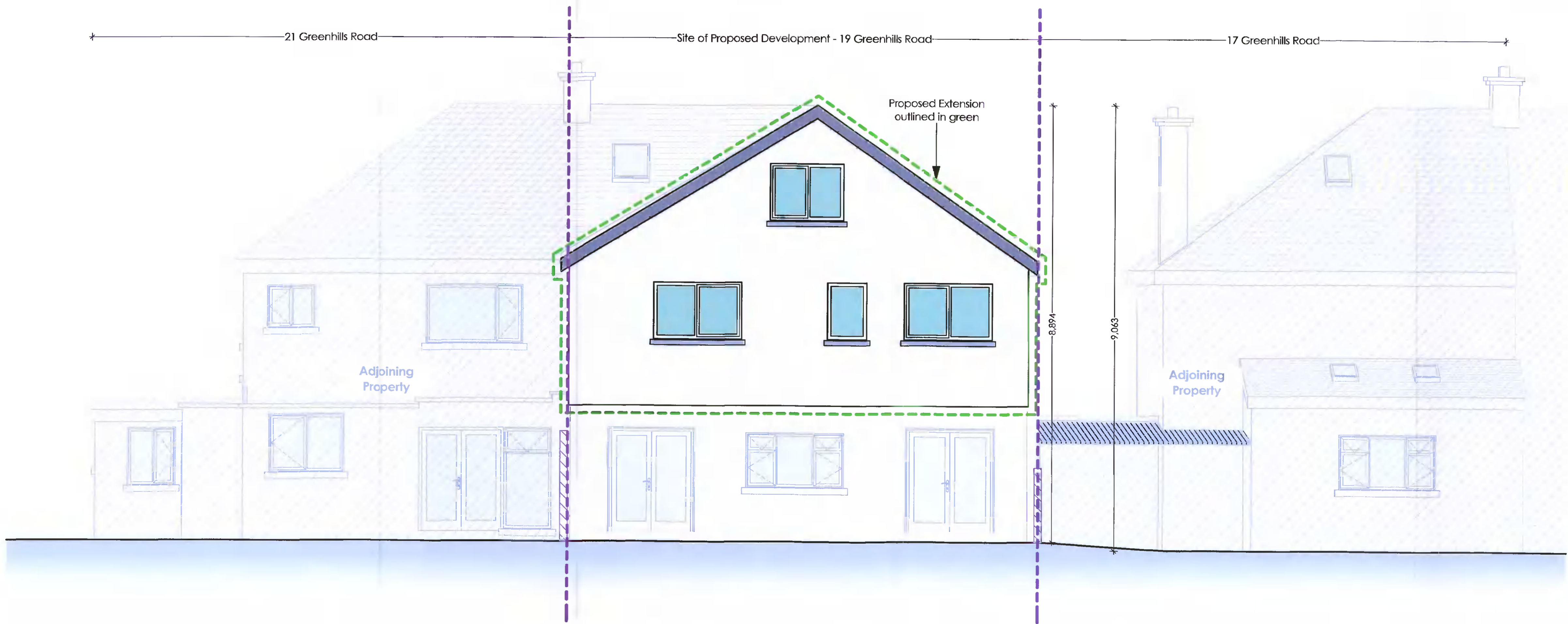
Proposed Contiguous Elevation - Southeast 1:100
