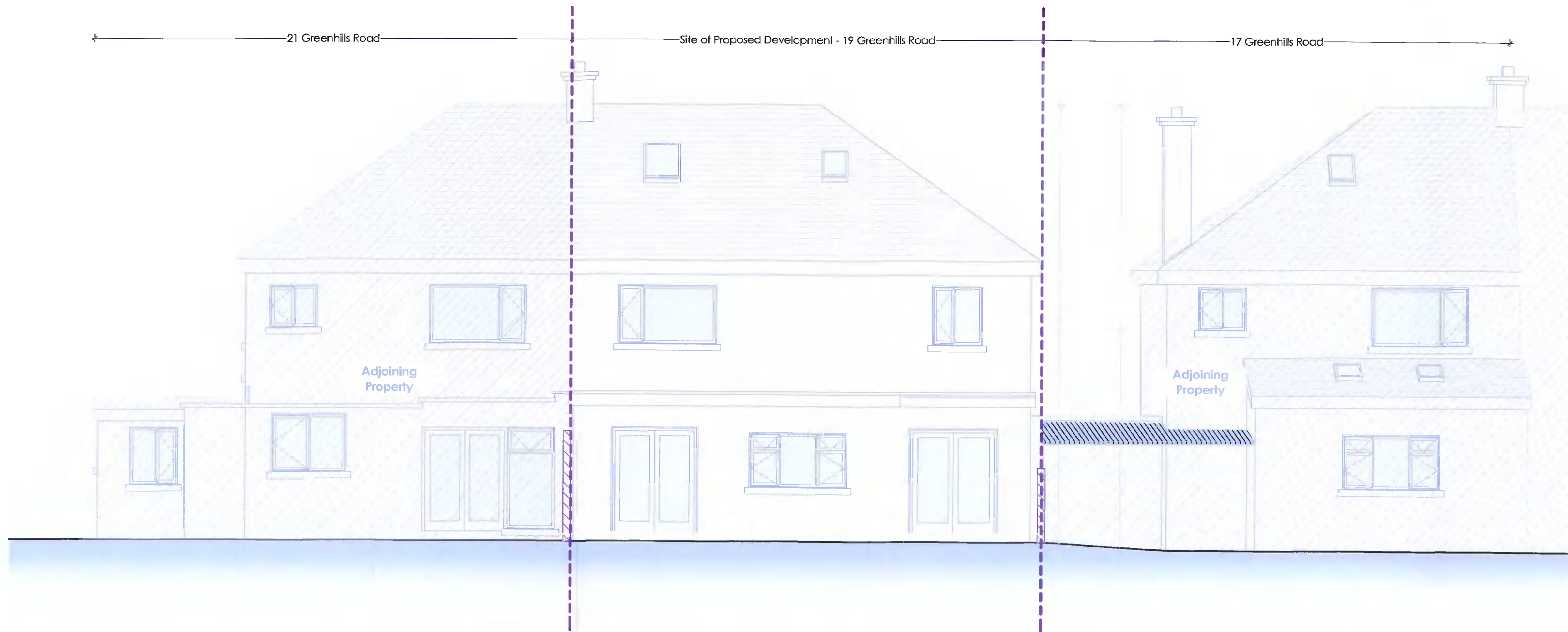
Existing Contiguous Elevation - Southeast 1:100
