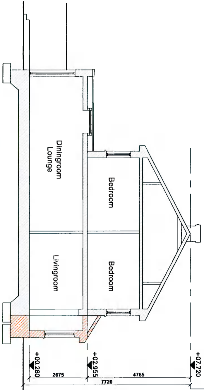
Proposed Section B-B Scale 1/100
