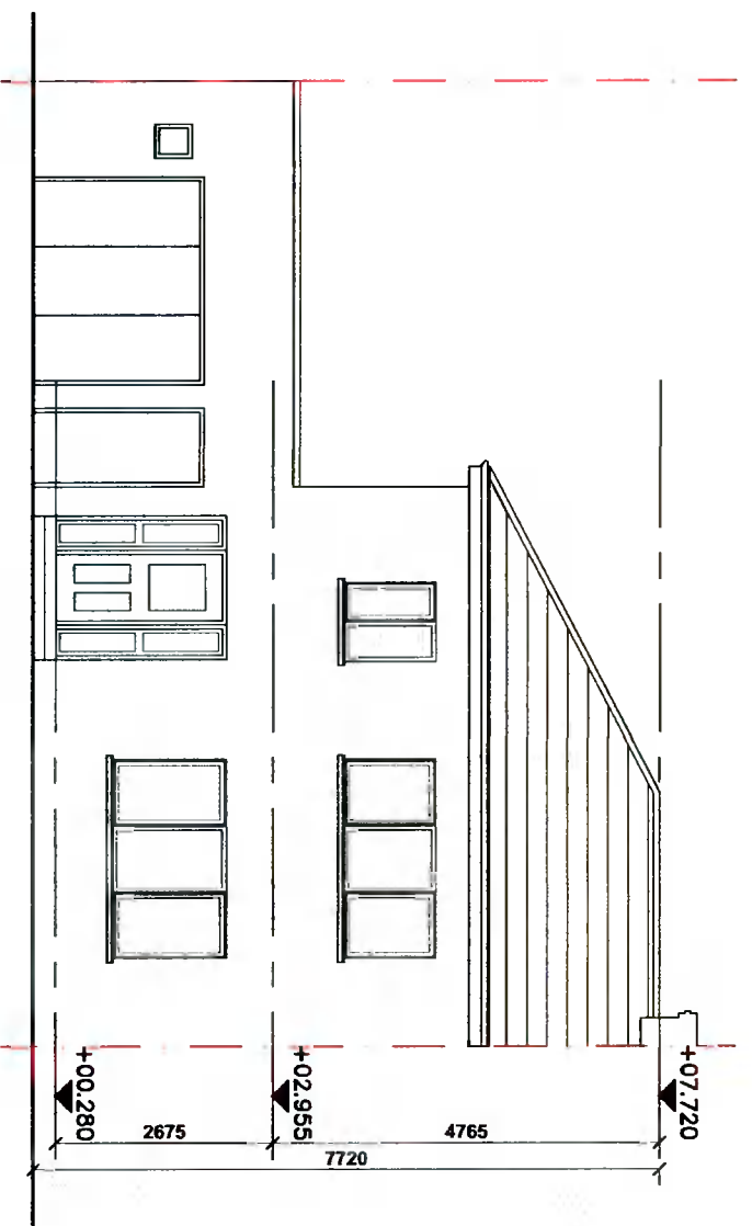
Existing Front Elevation Scale 1/100
