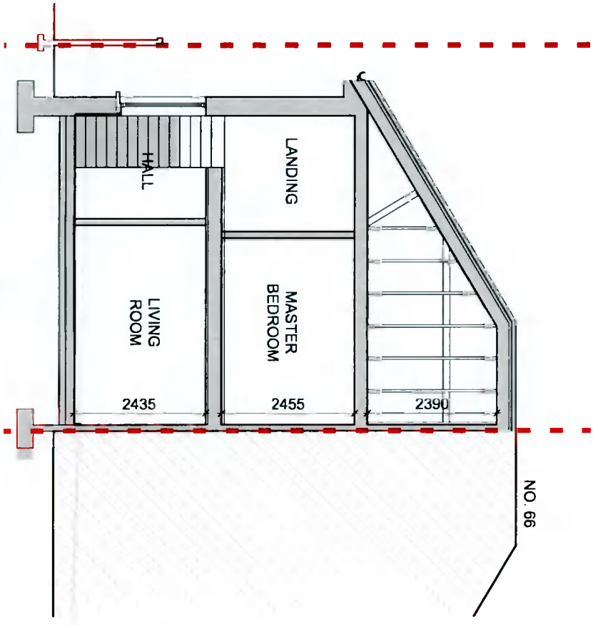
SECTION BB (existing)
