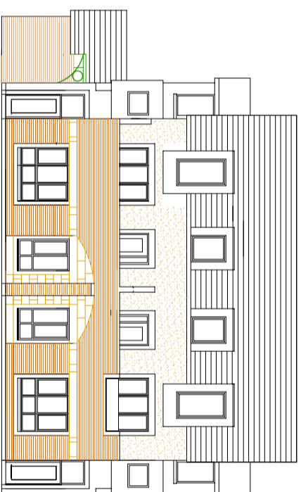
West elevation
