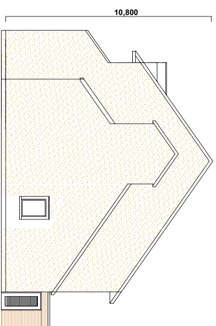
South elevation
