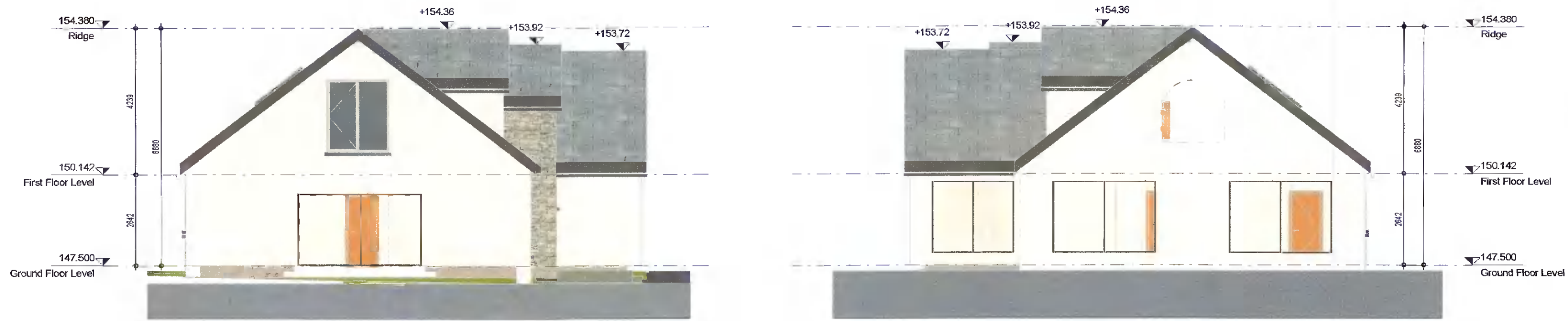
1 Existing/Demolition North East Elevation 1 : 100
