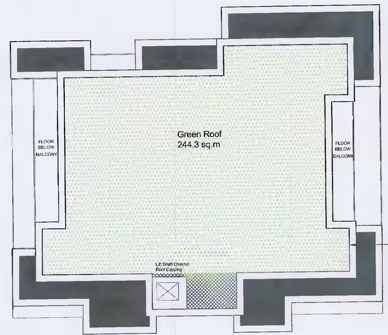
ROOF LAYOUT PLAN SCALE 1:150
