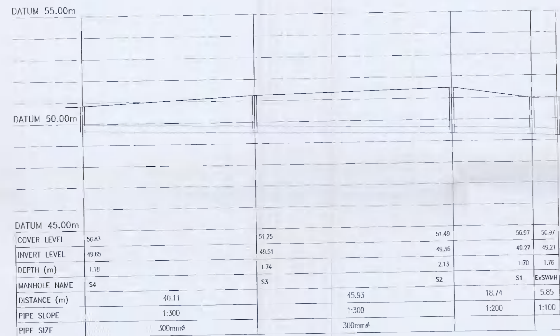
LONGITUDINAL SECTION (S4 to ExSWMH)
