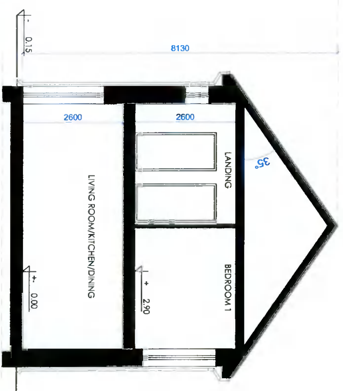
SECTION A-A- house type B1
