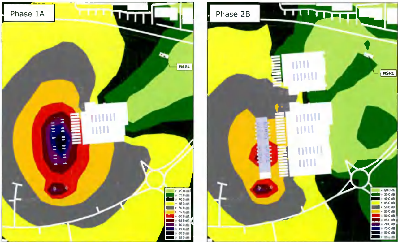
Figure 8-2: Overview of modelled noise emissions during normal operation.
