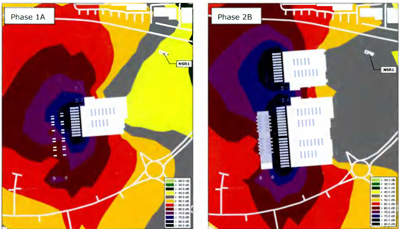
Figure 8-3: Overview of modelled emergency noise emissions.
