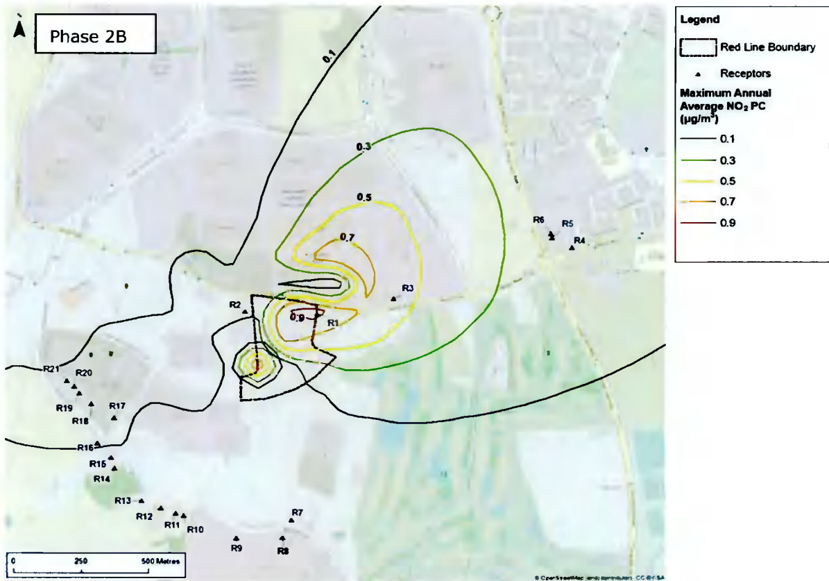
Figure 8-1: Phase 1A and Phase 2B Maximum Annual Average NO 2 PC (µg/m 3 ).
