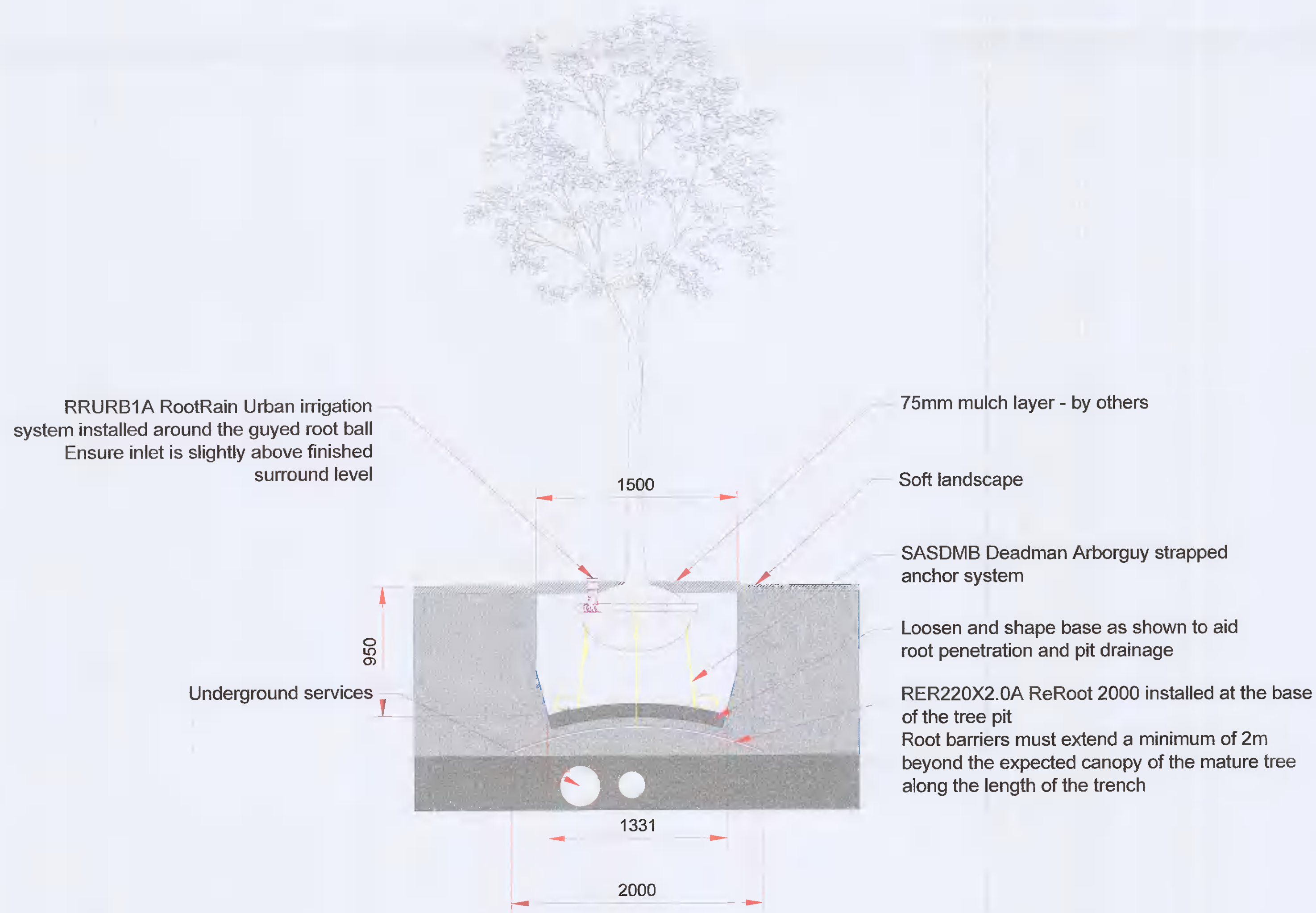
GreenBlue Urban 2102 Tree Pit System 1:25
