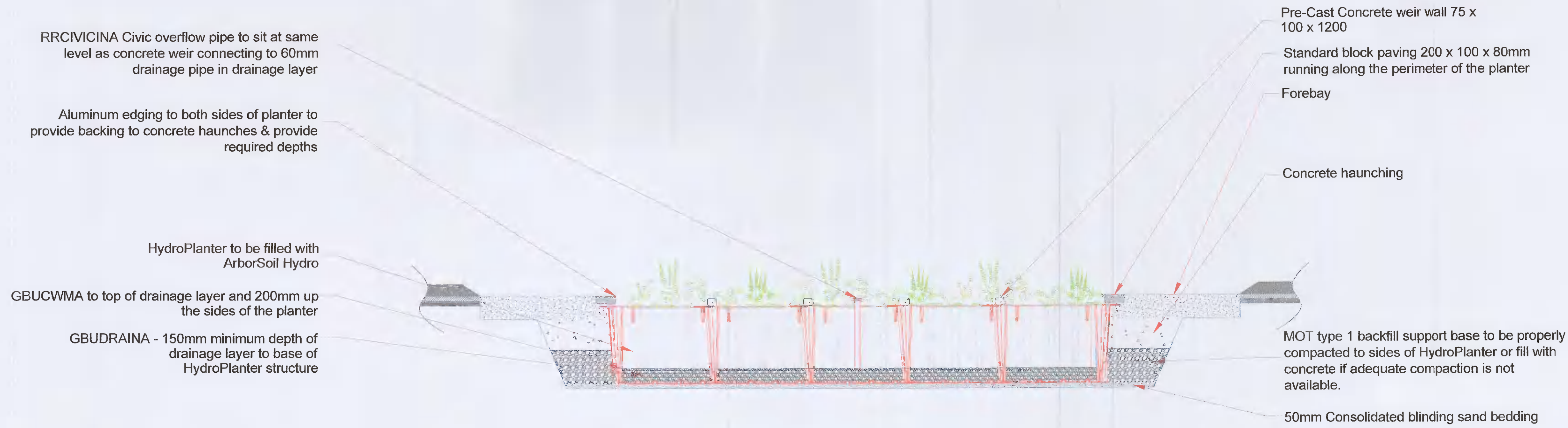
GreenBlue Urban 2121 HydroPlanter Rain Garden Product 1:25
