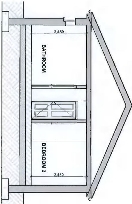
Section B-B (Existing) 1:100
