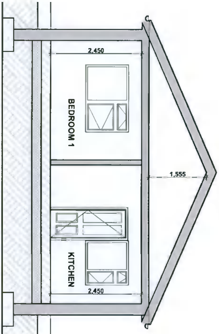
Section C-C (Existing) 1:100
