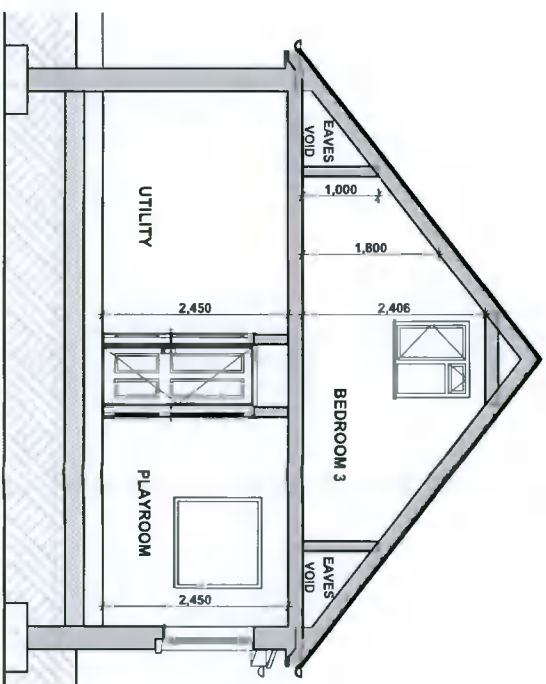
Section C-C (Proposed) 1:100
