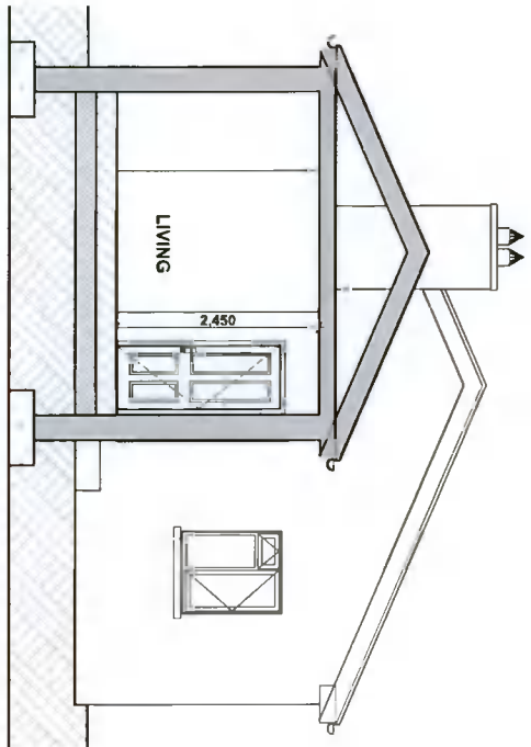
Section A-A (Existing) 1:100
