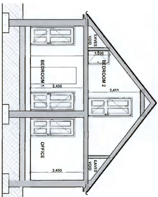
Section A-A (Proposed) 1:100
