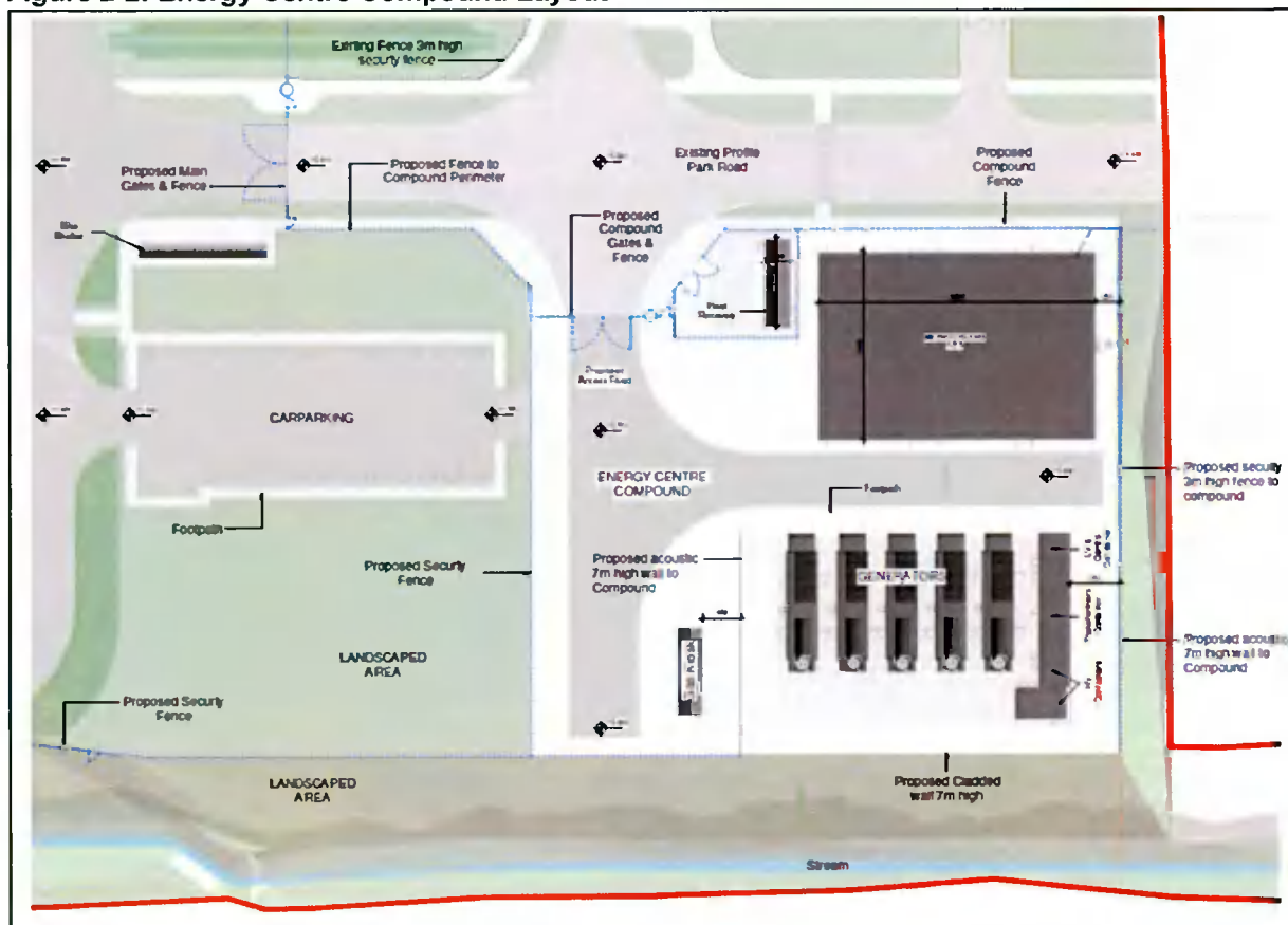
Figure 2-2: Energy Centre Compound Layout
