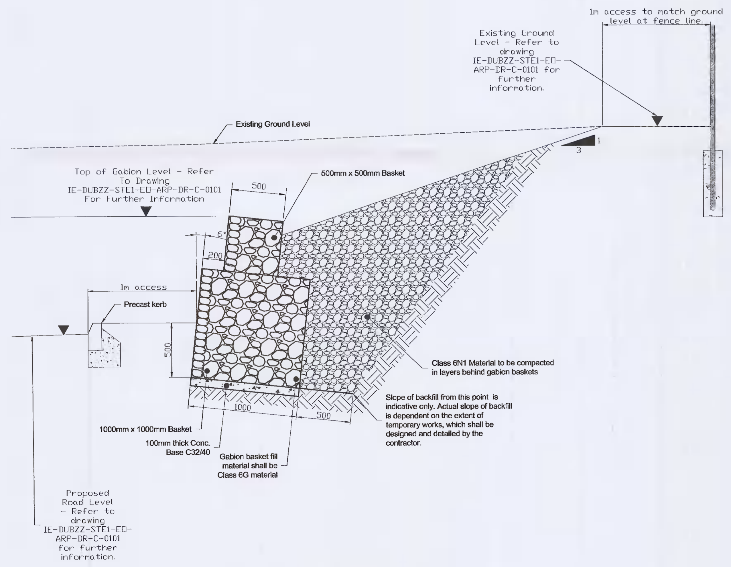
Proposed Gabion Basket Detail A Scale: 1:20
