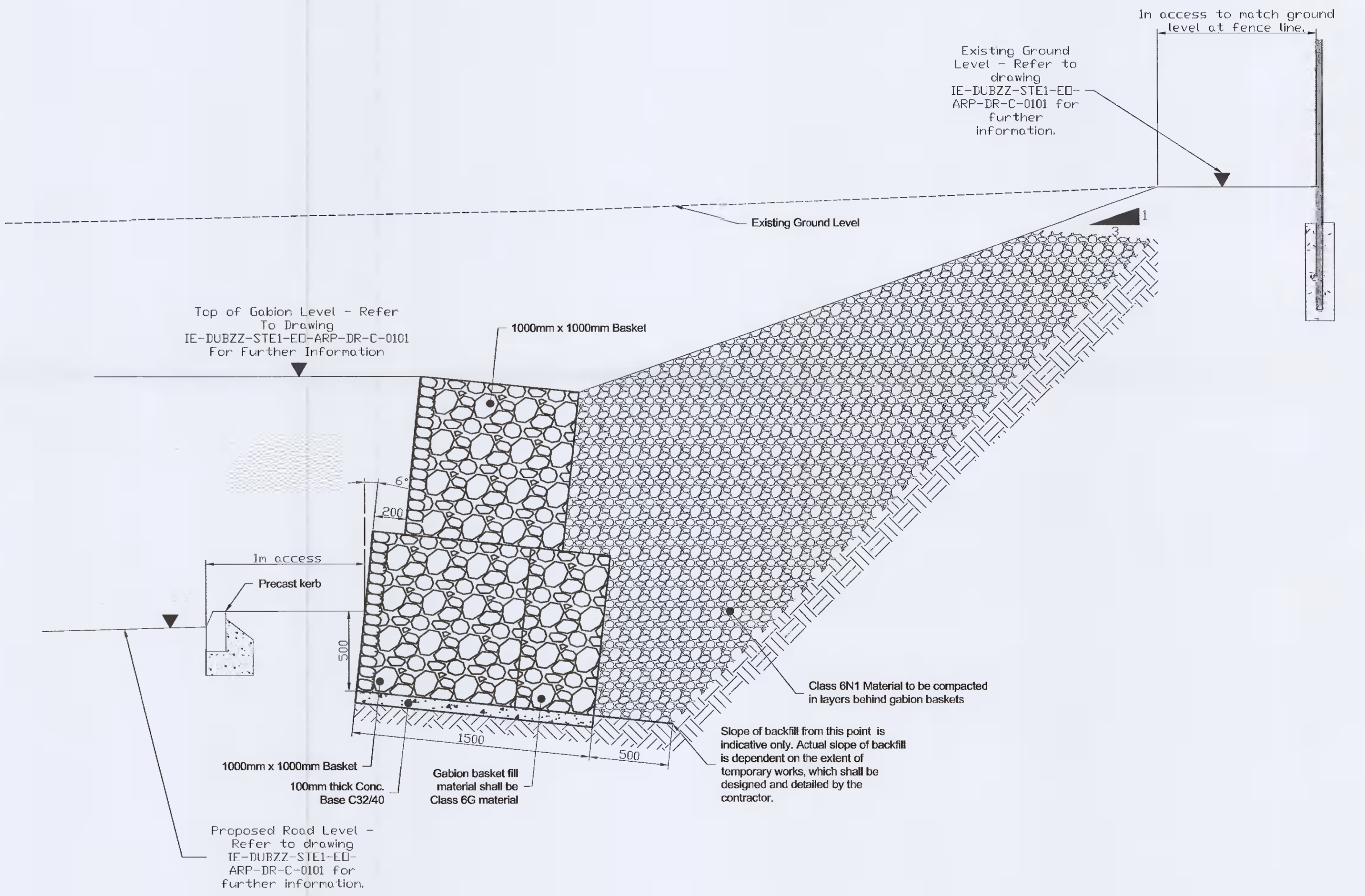
Proposed Gabion Basket Detail B Scale: 1:20
