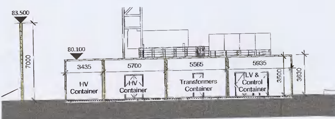
6 03023 Generator Compound - Section 1 : 200
