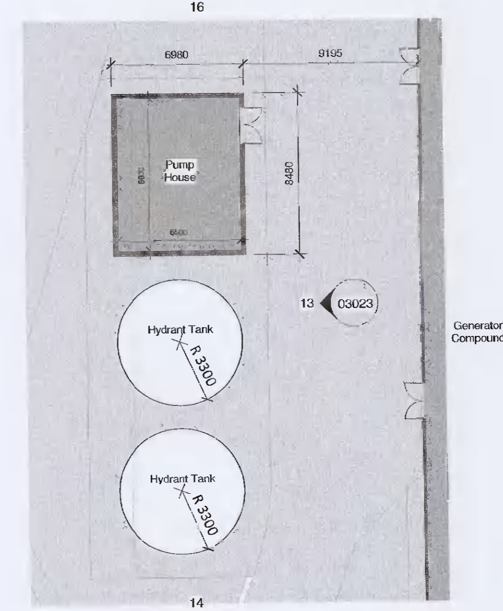
12 03023 Pump House - Ground Floor Plan 1 : 200
