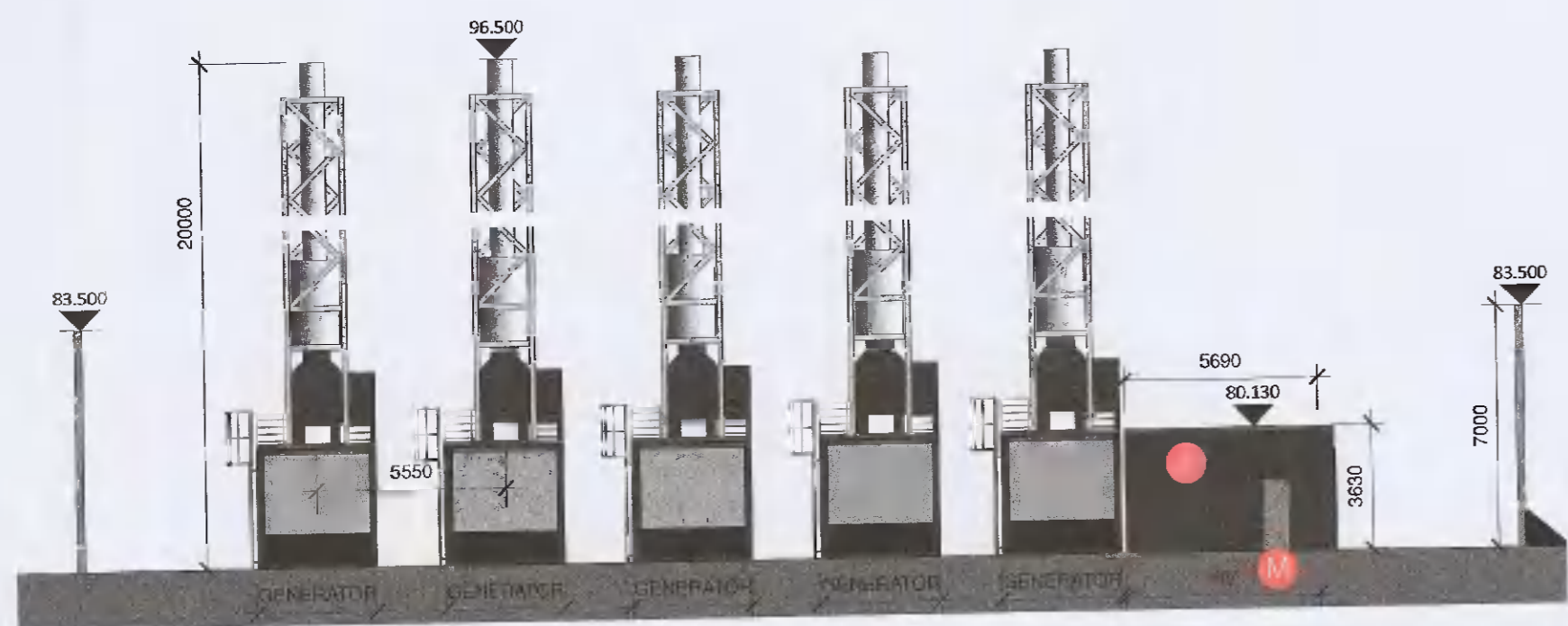
2 03023 Generator Compound - East Elevation 1 : 200
