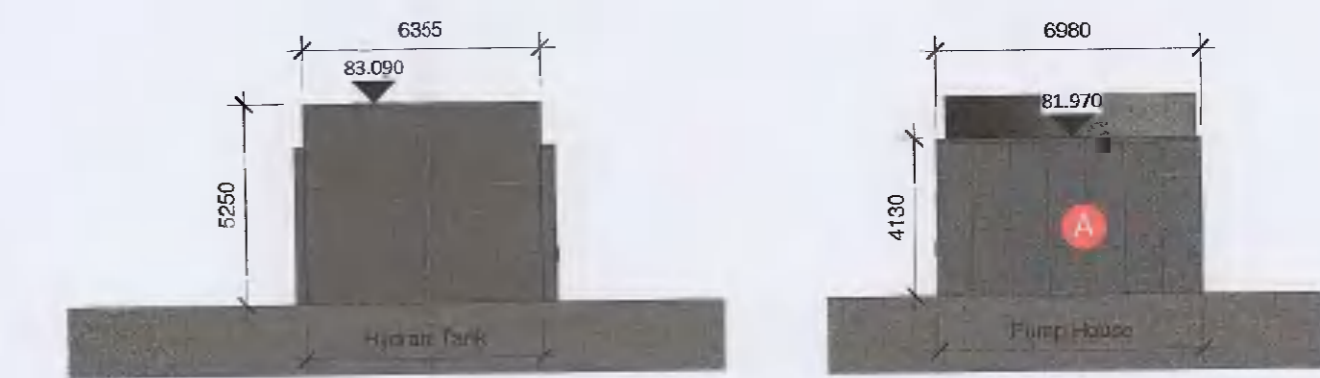
14 03023 Pumphouse - East & West Elevation 1 : 200
