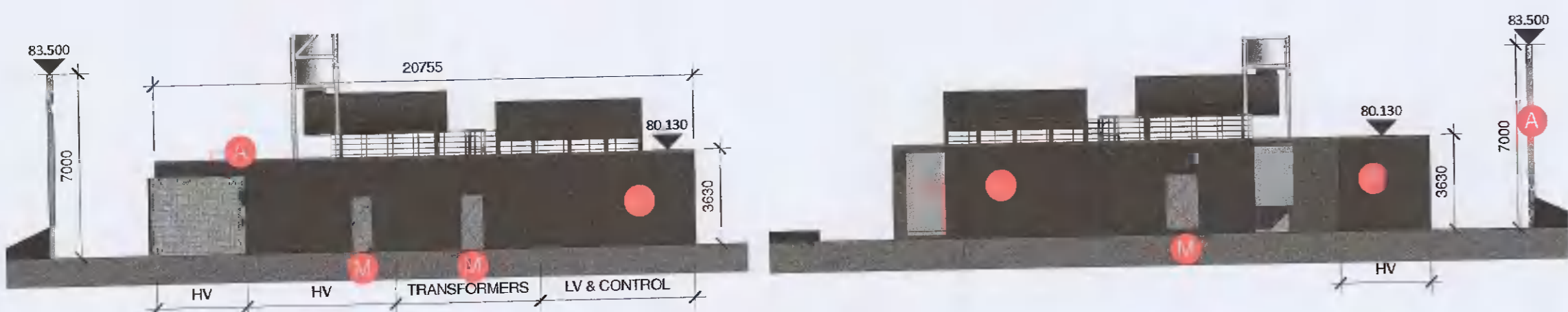
4 03023 Generator Compound - North & South Elevation 1 : 200
