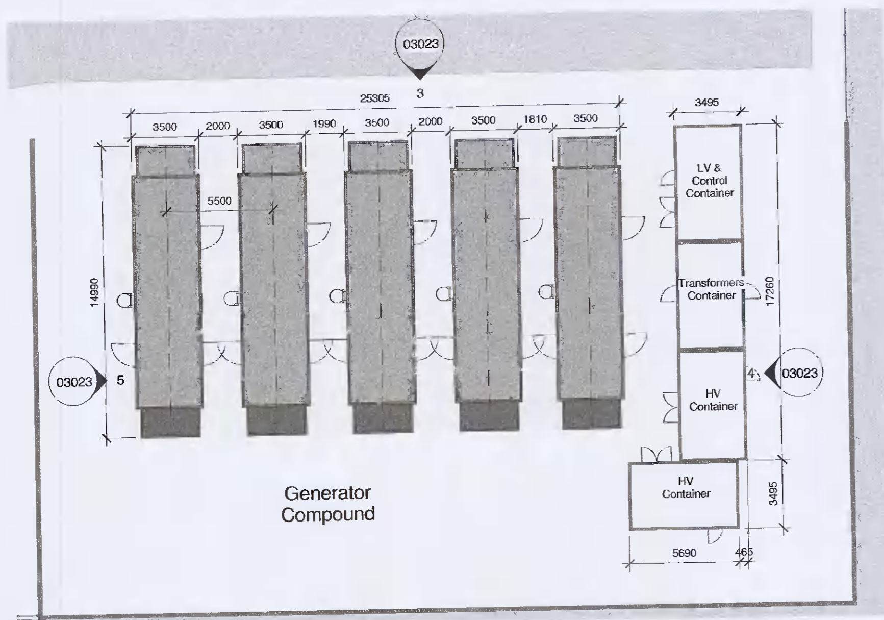
1 03023 Generator Compound - Ground Floor Plan 1 : 200
