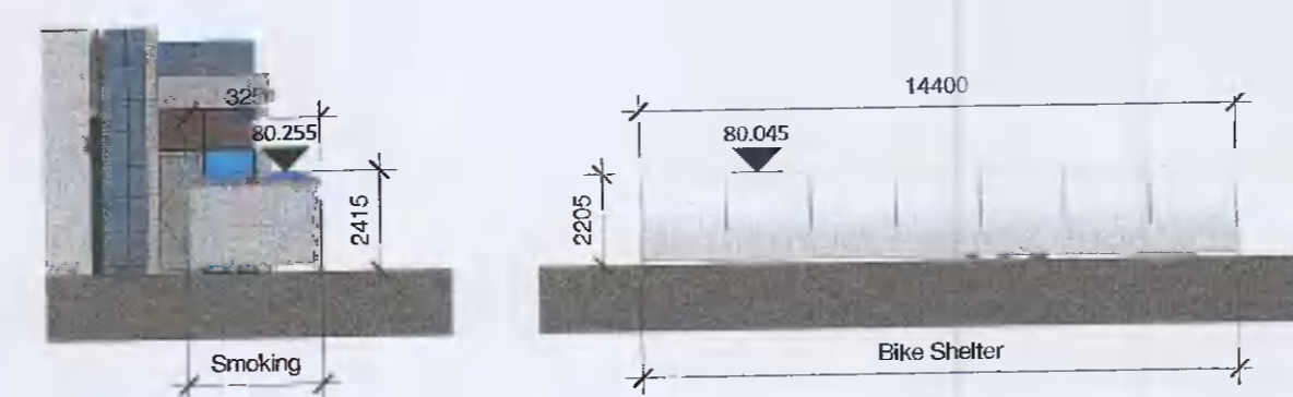
10 03023 Bike & Smoking Shelter - East Elevation 1 : 200
