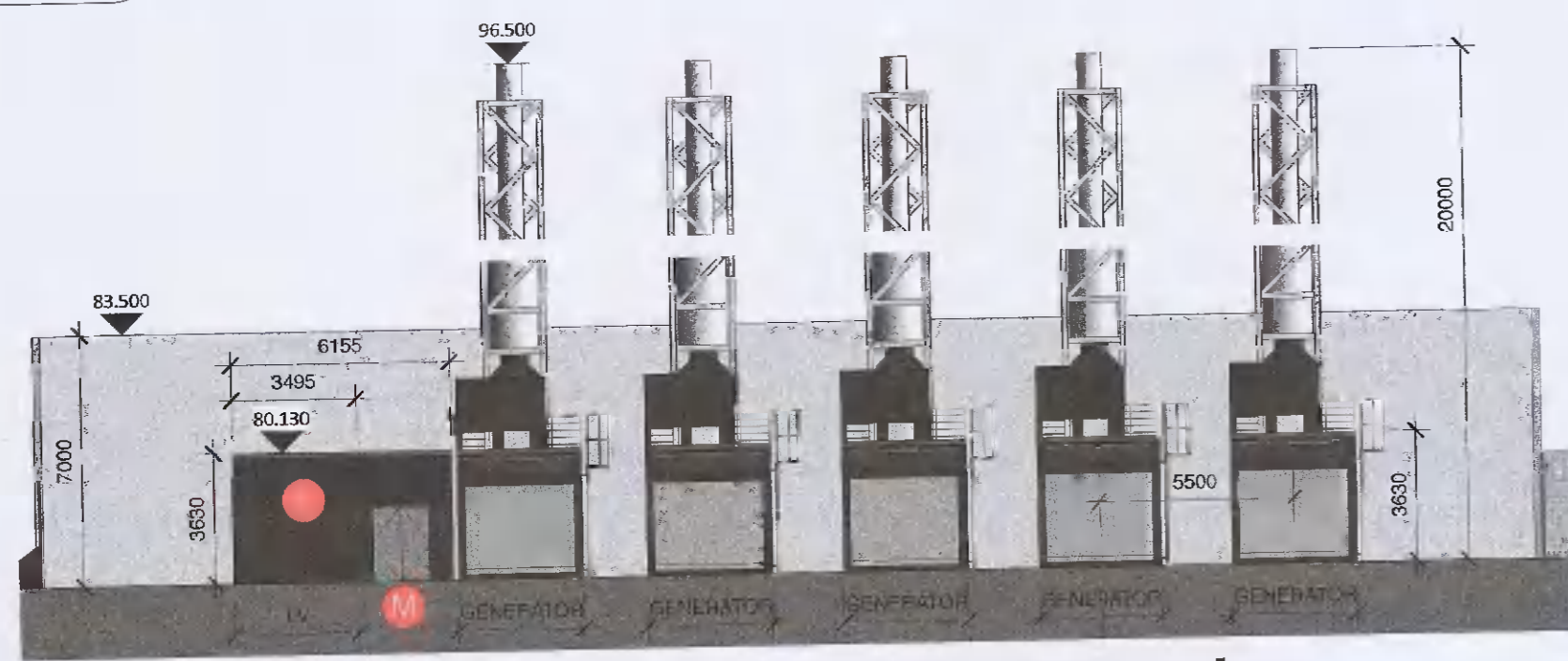
3 03023 Generator Compound - West Elevation 1 : 200
