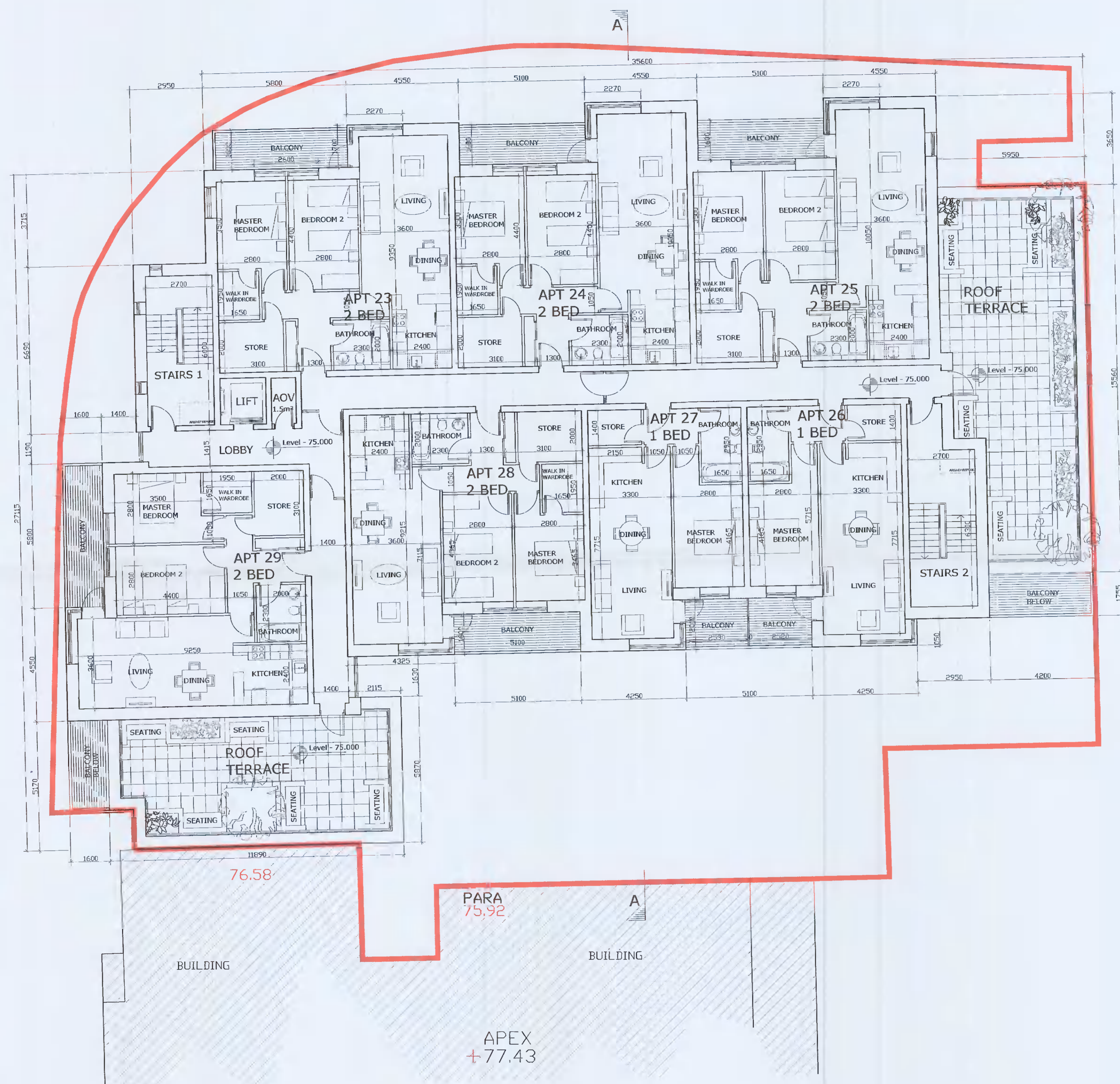
Proposed 3rd Floor Plan Scale 1:100 A1, 1:200 A3
